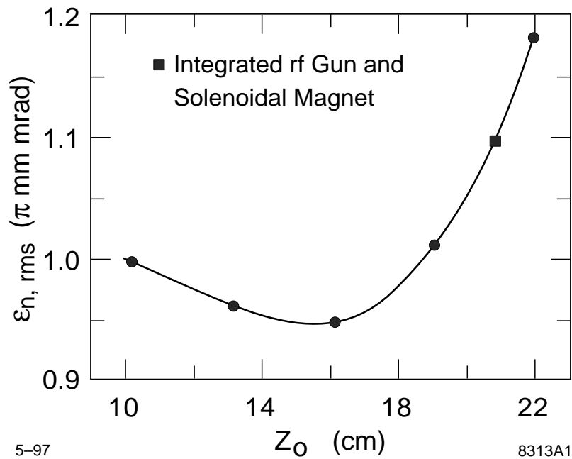
Figure 5. PARMELA simulation of compensated normalized emittance of ATF gun and beamline as a function of position (defined as the center) of the emittance compensating solenoid. The actual position of the solenoid during the experiments is shown by the square data point.
