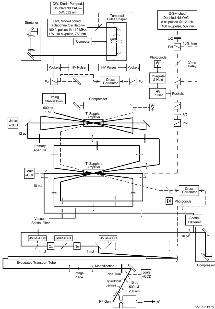
Figure 2. The drive laser for the rf photocathode electron gun for the LCLS. The thick lines show the main beam path, the closely spaced, dashed lines indicate diagnostic beams, and the widely spaced, dashed lines are pump beams.
