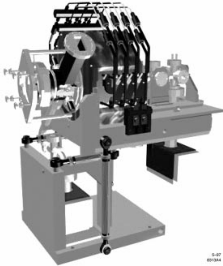
Figure 1. Perspective of the gun assembly. The beam exits to the right. ( Figure by C. Stelmach and S. Pjerov, NSLS, BNL).
