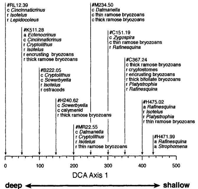
FIGURE 3 —Typical sample compositions from selected points along axis 1. Relative abundance coded as a (abundant), c (common), and r (rare); see text for explanation of these classes.
