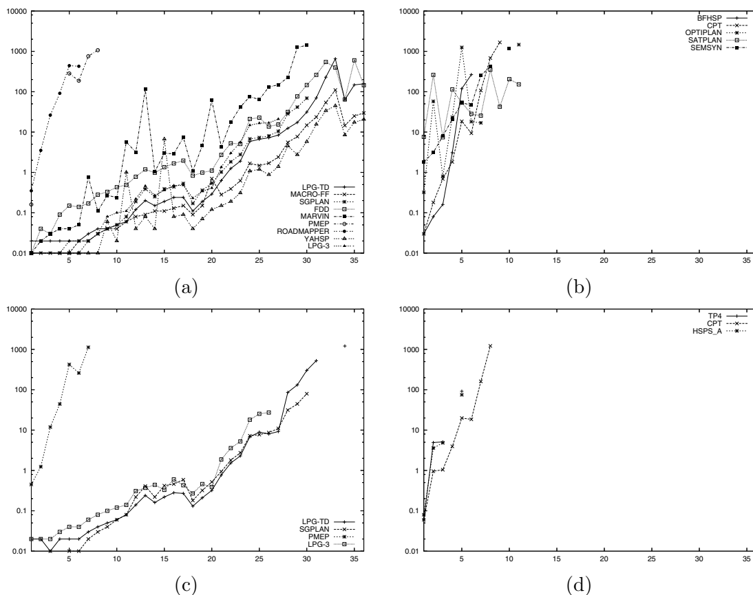
Figure 10: Satellite; Strips satisfying (a), optimal (b), and Time satisfying (c), optimal (d).
