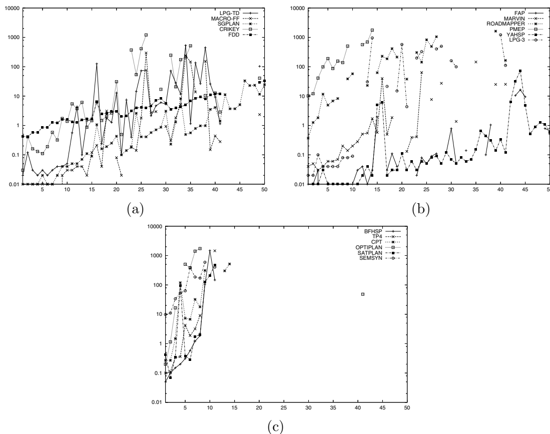
Figure 3: Non-temporal Pipesworld, no tankage constraints, satisfying (a) and (b), optimal (c).
