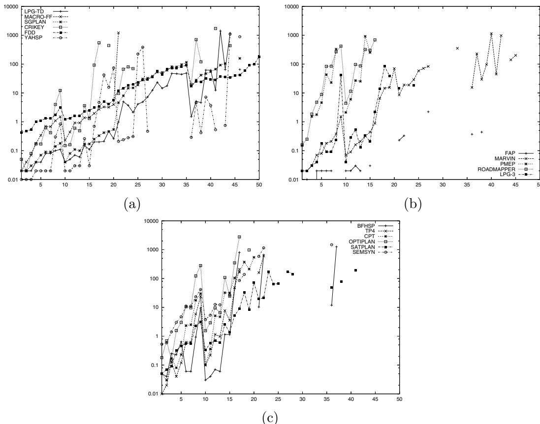
Figure 1: Performance in non-temporal Airport, satisficing (a) and (b), optimal (c).
