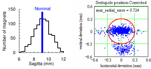
Fig. 21. Sagitta of the cold masses (left) and position of the correctors (right).
