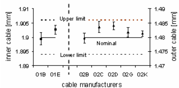
Fig. 18. Dimension of the cable during the production.
