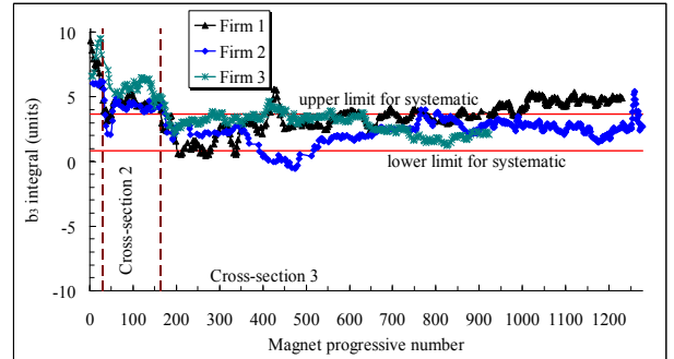
Fig. 25. Evolution of b_3 measured in aperture one during the production of 1276 dipoles, separated by assembler (warm magnetic measurements in the cold mass, running average of 5 magnets per firm). The target limits for the global average are shown in red.
