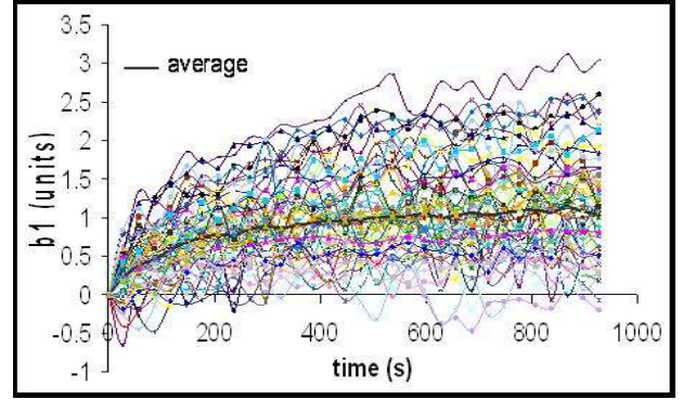
Fig. 33. Measured decay of the main field during the injection plateau measured in 35 LHC dipoles manufactured with cable of producer B [63].
