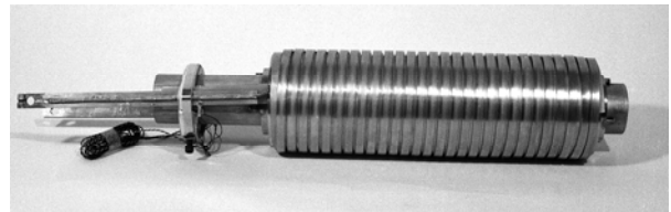
Fig. 6. A very early one-foot model magnet using spiral-wound stainless steel banding in two oppositely wound layers.
