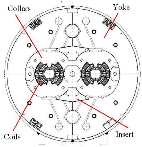
Fig. 15. Cross-section of the LHC dipole cold mass.
