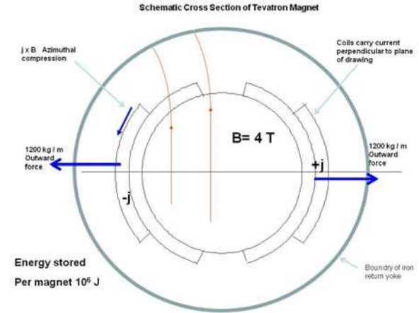
Fig. 1. Schematic drawing of the Tevatron dipole magnet transverse cross-section showing the configuration of the coil and iron return yoke as well as the direction of some of the forces acting on the coil.
