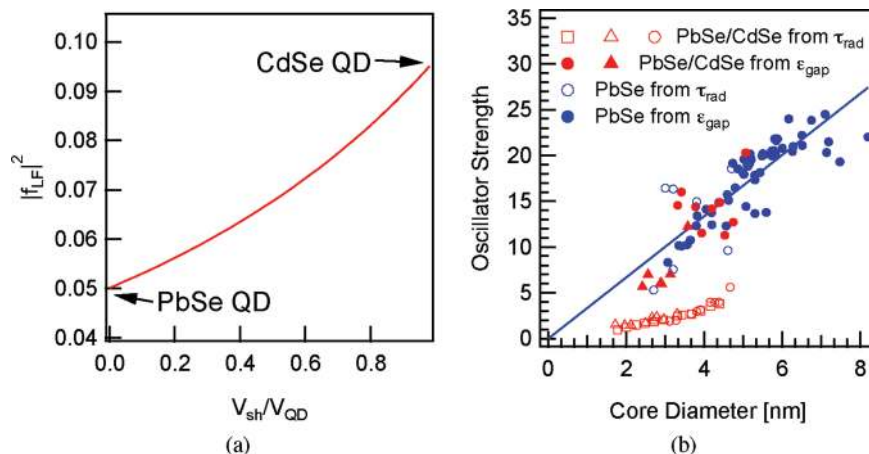
Figure 3. (a) Local field factor at the band edge for PbSe/CdSe QDs as a function of the ratio V_{\text{sh}}/V_{\text{QD}} . (b) Absorption oscillator strength f_{\text{if,abs}} for PbSe QDs (full blue markers) and PbSe/CdSe QDs (full red markers) and emission oscillator strength f_{\text{if,em}} for PbSe QDs 14,15 (empty blue markers) and PbSe/CdSe QDs (empty red markers) as a function of the core diameter. Shown are the values for PbSe/CdSe with a total diameter of (red squares) 6.09 nm, (red dots) 5.83 nm, and (red triangles) 4.57 nm. The full red curve is a Boltzmann model of the emission oscillator strength for two states separated by the experimentally determined Stokes shift.
