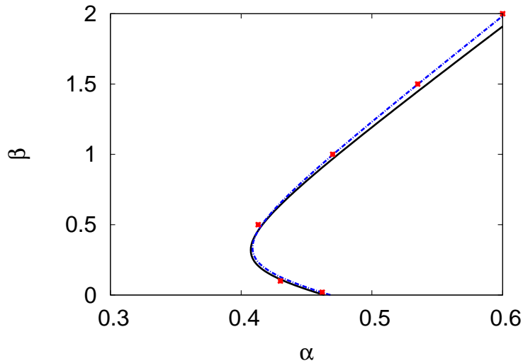
Figure 5: The regions of the \alpha - \beta plane in which Hopf bifurcation can occur for the 1-D spatial domain. The one-term (black solid line), the two-term (blue, dashes) regions and the numerical solution (red, squares) are shown. The other parameters are \gamma_1 = 0.1 , D_1 = D_2 = 0.1 , \delta_1 = 0.2 , \gamma_2 = 0.7 , \delta_2 = 0.5 and \tau_1 = \tau_2 = 4 .
