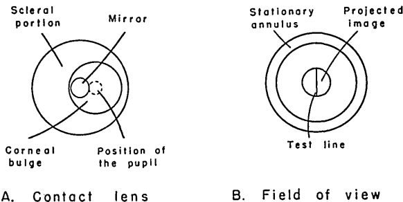
FIG. 1. A, The contact lens used in the present experiment. B, The appearance of the visual field.
