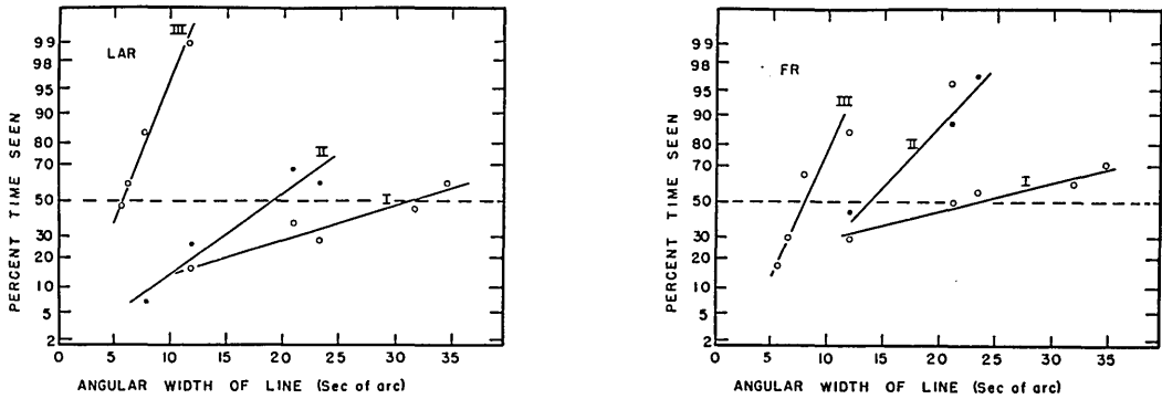
FIG. 3. Percent time seen as a function of width of line for one-minute exposures, subjects LAR and FR. Condition I is the condition in which the effects of eye movements were "compensated," Condition II "normal," and Condition III "exaggerated."
