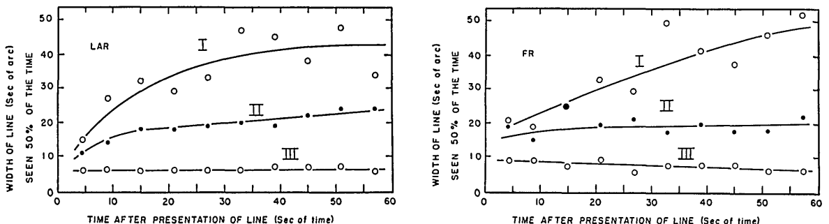
FIG. 4. Width of line seen 50 percent of the time during successive sections of the one-minute interval under viewing Conditions I, II, and III, subjects LAR and FR.
