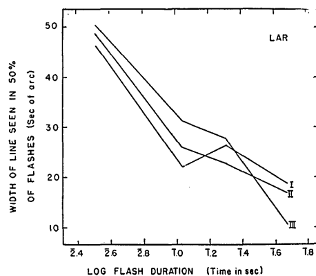
FIG. 5. Width of line seen in 50 percent of flashes as a function of flash duration under viewing Conditions I, II, and III, subject LAR.
