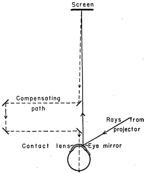
FIG. 2. Diagram of the method for counteracting the effects of eye movements. The viewing path is effectively double the distance from the eye to the screen. The compensating path includes two dove prisms and an arrangement for providing fixation at the center of a bright annular field.
