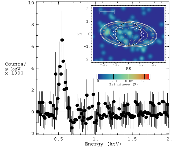
FIG. 4.—Background-subtracted energy spectrum for ring X-ray emission during the Chandra ACIS 2003 April 14–15 observation (Ness et al. 2004). A cluster of X-ray photons in the \sim 0.49 – 0.62 keV band around the 0.53 keV oxygen K\alpha line is clearly evident in the spectrum. Note that the energy resolution of ACIS-S3 at these energies is \sim 120 eV. The inset shows the Chandra ACIS X-ray image of the Saturn system in the 0.49–0.62 keV band on 2003 April 14–15. The description of this figure is the same as for Fig. 1. The rings’ X-ray emission is evident on the east ansa (morning) in this image, which is also mentioned by Ness et al. (2004).
