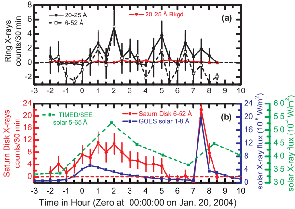
FIG. 3.—X-ray light curve for Saturn’s rings and disk and the Sun on 2004 January 20. All data are binned in 30 minute increments, except for the TIMED/SEE data, which are 3 minute observation-averaged fluxes obtained every orbit ( \sim 12 measurements per day). (a) Background-subtracted ring X-ray emission in 0.24–2.0 and 0.49–0.62 keV bands observed by Chandra ACIS, plotted after shifting by -2.236 hr to account for the light-travel time difference between Sun-Saturn-Earth and Sun-Earth. Expected background in the 0.49–0.62 keV band is shown in red. (b) Background-subtracted Saturn disk 0.24–2.0 keV emission (there are only six events in the 0.49–0.62 keV band from the disk) plotted in red after shifting by -2.236 hr. The solar X-ray flux in the 1.6–12.4 keV band measured by the Earth-orbiting GOES-12 is plotted in blue. The solar 0.2–2.5 keV fluxes measured by TIMED/SEE are solid green squares and are joined by the green dashed line for visualization purposes. A flare in the light curve for Saturn’s disk and for the solar X-ray flux is observed at about 7.5 hr. Although the light curve for ring X-ray emission is somewhat similar to that for the disk X-ray emission, no flaring is evident.
