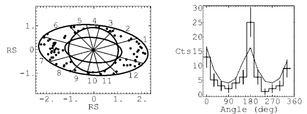
FIG. 5.—Distributions of X-ray events in the 0.49–0.62 keV band from the rings of Saturn obtained by combining the 2004 January and 2003 April Chandra ACIS observations. Left : Distribution in the ring plane in 30^\circ -wide sectors, with sector 1 ranging from -15^\circ to +15^\circ in azimuthal angle measured from the horizontal axis. Diagonally opposite sectors have equal area. Right : Distribution of counts in the 30^\circ sectors of the left panel. The dotted curve shows the distribution expected if the emission from each sector were proportional to its area, normalized so that the total number of photons equals what is observed.
