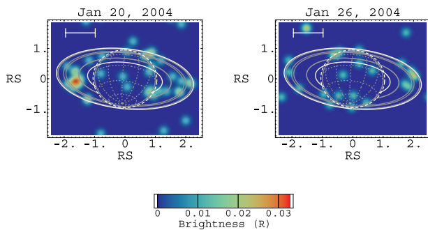
FIG. 1.— Chandra ACIS X-ray images of the Saturnian system in the 0.49–0.62 keV band on 2004 January 20 and 26–27. The X-ray emission from the rings is clearly present in these restricted energy band images (see Fig. 2); the emission from the planet is relatively weak in this band (see Fig. 1 of Bhardwaj et al. 2005a for an X-ray image of the Saturnian system in the 0.24–2.0 keV band). The false-color images, with brightness in rayleighs (R), show X-ray photons as seen in a frame moving across the sky with Saturn, smoothed with a two-dimensional Gaussian with \sigma = 0''.984 (twice the ACIS pixel width). For the conversion to rayleighs, we used a value for effective area of 195 \text{ cm}^2 at 0.525 keV—the energy of the atomic oxygen K\alpha emission line. The horizontal and vertical axes are in units of Saturn’s equatorial radius (RS). The white scale bar in the upper left of each panel represents 10'' . The superposed graticule shows latitude and longitude lines at intervals of 30^\circ . The solid gray lines are the outlines of the planet and rings, with the outer edge of the A ring and inner edge of the C ring shown in white. The dotted white line defines the region within which events were accepted as part of Saturn’s disk, unless obscured by the rings. The two images, taken a week apart and shown on the same color scale, indicate substantial variability in X-ray emission from the rings.
