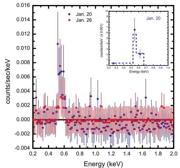
FIG. 2.—Background-subtracted Chandra ACIS-S3-observed X-ray energy spectrum for Saturn’s rings in the 0.2–2.0 keV range on 2004 January 20 and 26–27. The cluster of X-ray photons in the \sim 0.49 –0.62 keV band suggests the presence of the oxygen K\alpha line emission at 0.53 keV in the X-ray emission from the rings. The inset shows a Gaussian fit (peak energy = 0.55 keV, \sigma = 140 eV), shown by the dashed line, to the ACIS-observed rings’ spectrum on January 20. Each spectral point (filled circle with error bar) represents \geq 10 measured events. The spectral fitting suggests that X-ray emissions from the rings are predominantly oxygen K\alpha photons.
