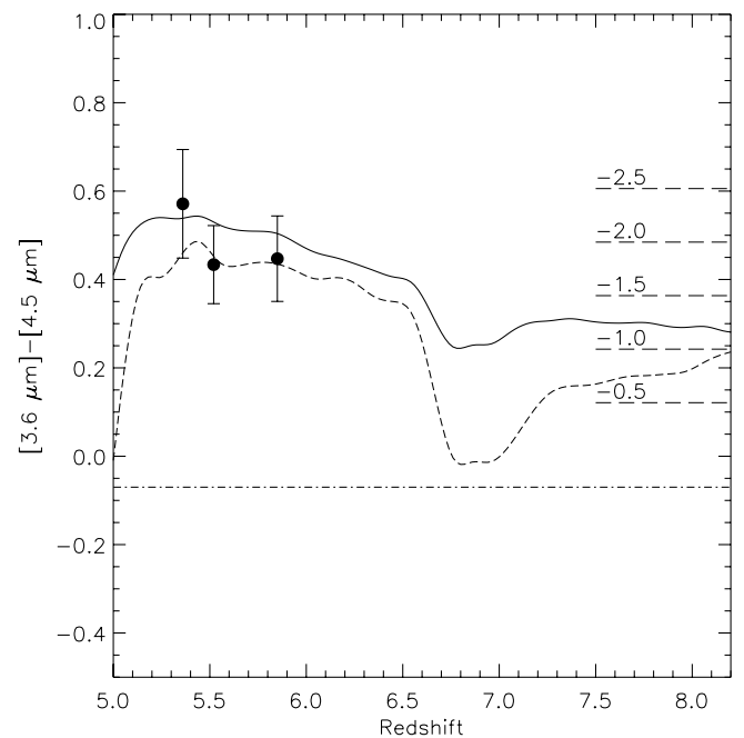
FIG. 7.—Plot of [3.6] - [4.5] color of quasars to very high redshift based on the SDSS quasar composite (solid line; Vanden Berk et al. 2001) or a \alpha_\nu = -0.5 power-law combined with the Balmer emission lines observed in the SDSS composite spectrum (dashed line). The color cut imposed by the mid-infrared selection of quasars in AGES is shown by the dot-dashed line. Longward of rest-frame 5000 Å, the SDSS composite is dominated by low-luminosity AGNs and is likely heavily contaminated by host-galaxy light, making the colors slightly redder. For comparison, the locations of the three z > 5 quasars discovered here are marked, and the dashed lines on the right mark the colors of pure power-law spectra with different values of \alpha_\nu . The rapid rise at z = 5 occurs as the H\alpha emission line passes from the 3.6 \mu\text{m} band into the 4.5 \mu\text{m} bandpass. Similarly, as the H\alpha emission line redshifts out of the 4.5 \mu\text{m} bandpass near z \sim 6.5 , the colors drop quickly; the colors become redder again near z \sim 7 as the H\beta enters the 4.5 \mu\text{m} bandpass. Even at very high redshifts, the colors of quasars predicted by both tracks fall within the region used for the mid-infrared selection of quasars in our survey.
