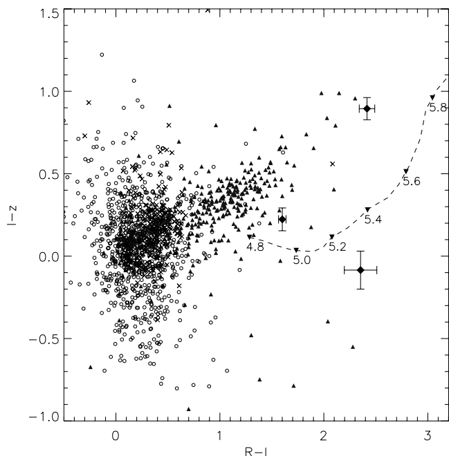
FIG. 4.—Optical color-color space for AGES point sources. The symbols are defined as in Figure 3. In addition, the dashed line shows the expected colors of quasars at z > 4.8 predicted using the SDSS quasar composite (Vanden Berk et al. 2001) modified by the addition of absorption blueward of Ly \alpha using the prescription of Songaila & Cowie (2002). The three high-redshift quasars discovered in this work occupy the same location in color-color space used in the past to optically select z > 4.5 quasars. At the same time, two of the three objects lie very near the stellar locus in this color-color space, illustrating one of the main difficulties in using optical colors alone to select high-redshift quasars. [See the electronic edition of the Journal for a color version of this figure.]
