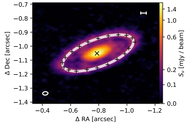
Figure 4. Fit of an ellipse to the AS 205 S ring in the outer disk. The plus symbols mark the maximum emission along the ring, while the white line shows the best fit. At the center, the black cross marks the best-fit center of the ellipse. The beam is given in the bottom-left corner, and a 5 au scale bar is in the upper-right corner for comparison.
