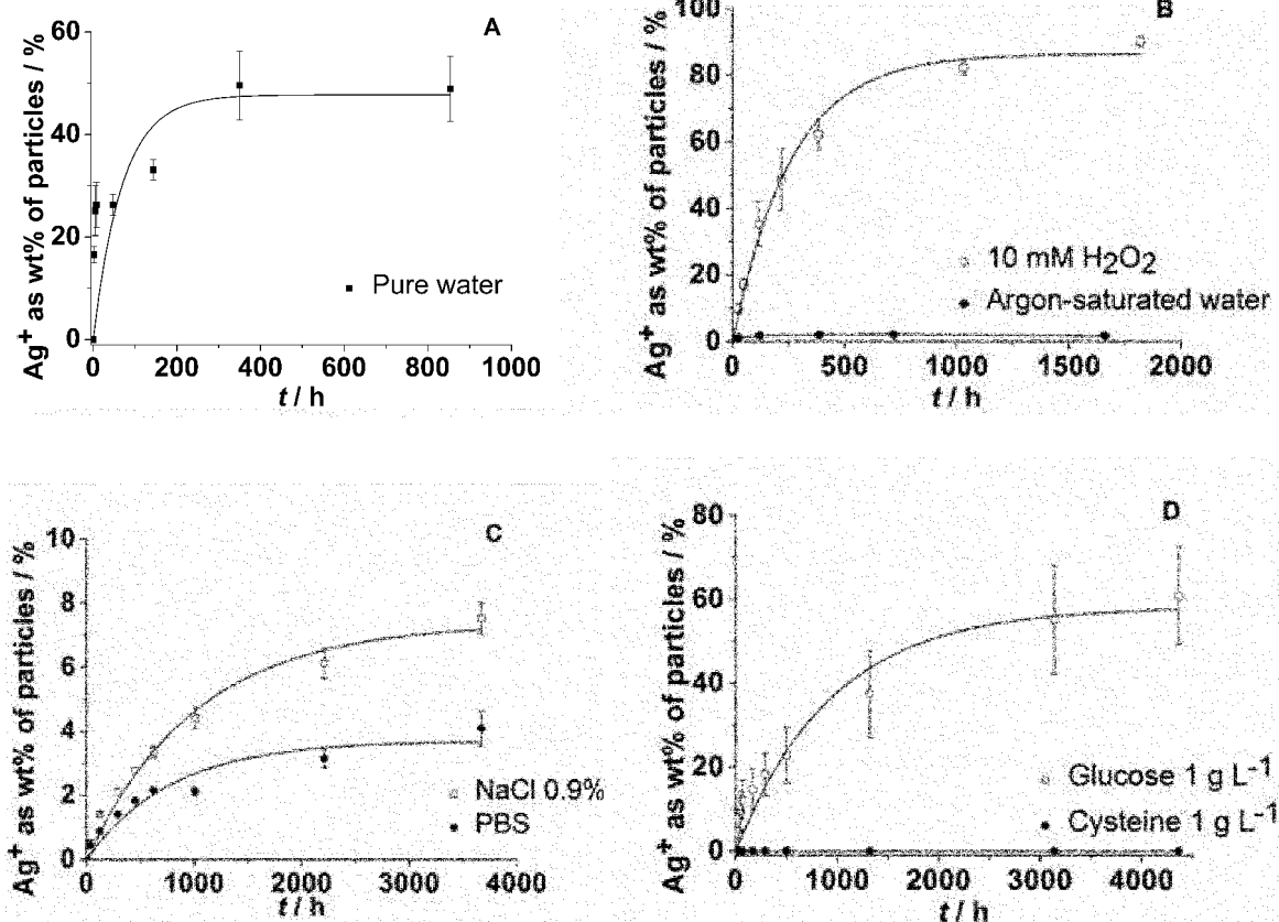
Fig. 1 Dissolution of silver nanoparticles immersed in pure water (A: data taken from ref. 15), degassed, argon-saturated water under an argon atmosphere, and in water with 10 mM \text{H}_2\text{O}_2 (B), in aqueous NaCl (0.9%) or in PBS (C), and in the presence of either cysteine (aq.: 1 \text{ g L}^{-1} ) or glucose (aq.: 1 \text{ g L}^{-1} ) (D).
