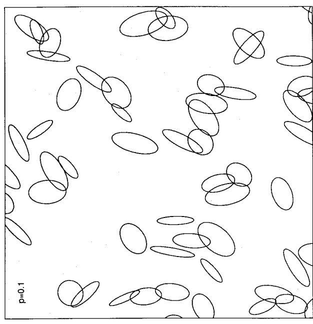
Figure 1. Polarization of a field of elliptical galaxies. The polarization, p , is uniform over the field. (a) p = 0.0 (– no effect), (b) p = 0.1 .
