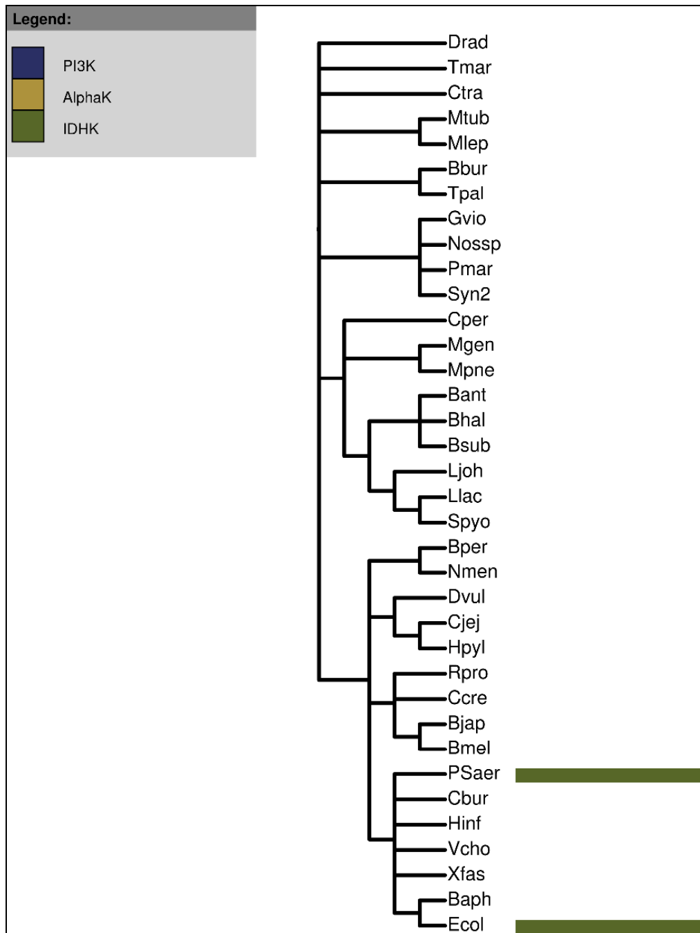
Figure 4.14 Bacterial IDHK family.
