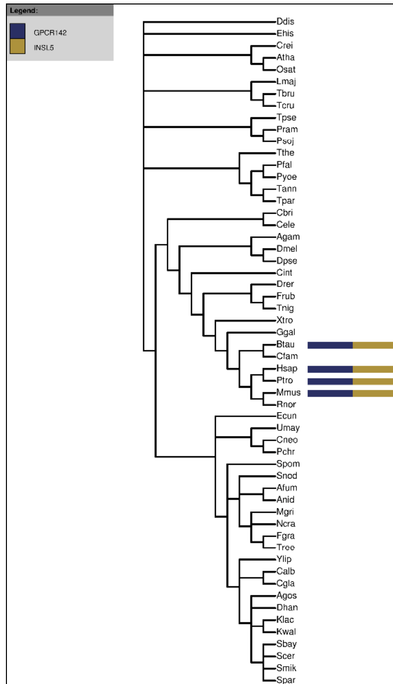
Figure 5.2 Eukaryotic GPCR142 and INSL5 families.
