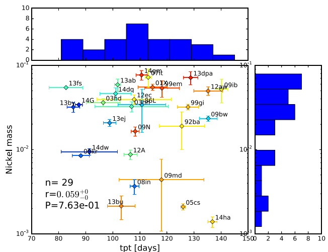
Figure 21. ^{56}\text{Ni} mass as a function of time of the transition between the plateau and radioactive tail; n is the number of events, r is Pearson’s correlation coefficient, and P is the probability of detecting a correlation by chance. The objects are colour-coded with respect to the V -band decline rate over 50 d ( s_{50V} ).
