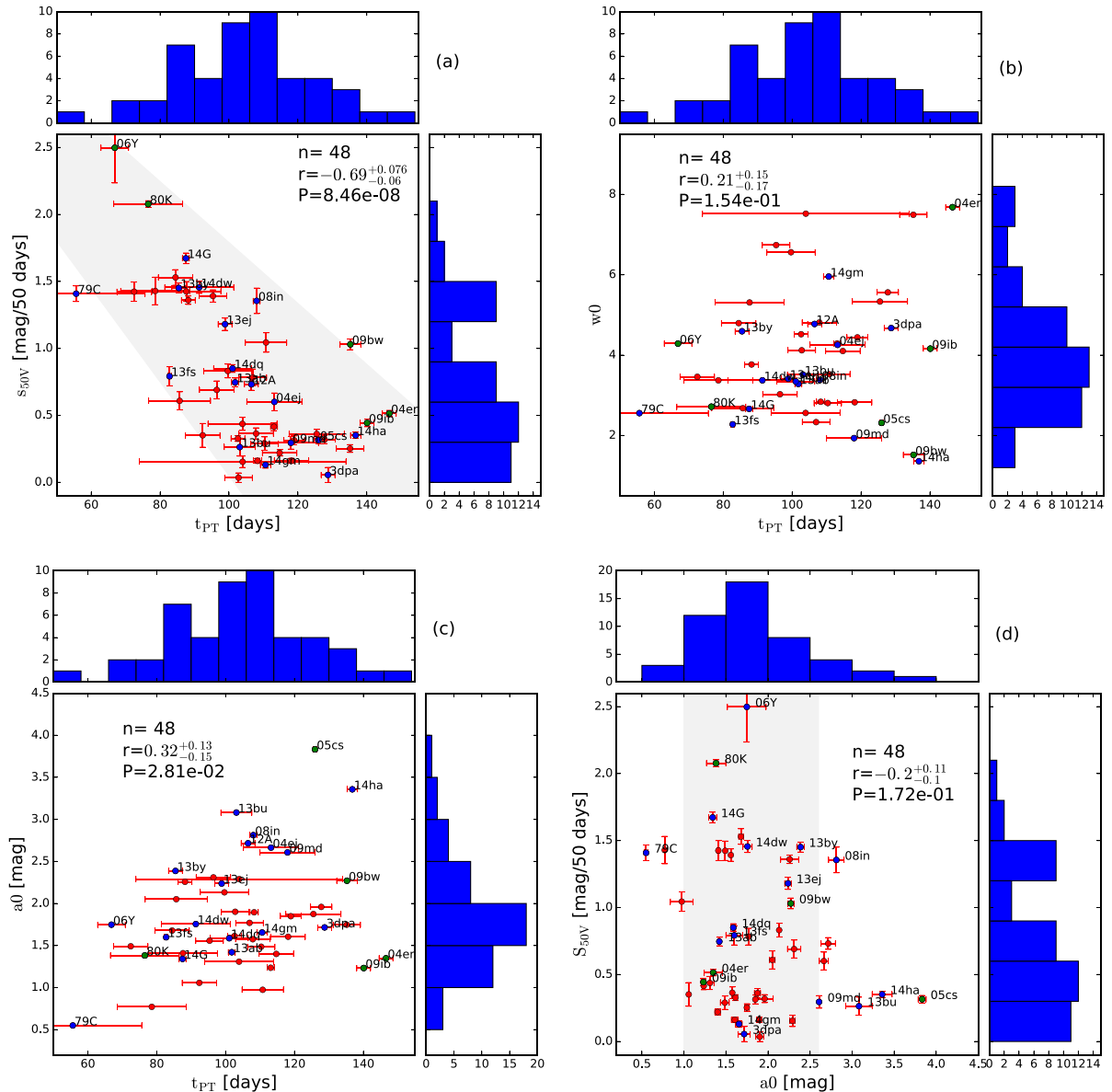
Figure 5. Correlation among s_{50V} , t_{PT} , w_0 , and a_0 , as obtained from V -band light curves. Our sample is marked in blue; some other SNe are highlighted in green. For each panel, n is the number of events, r is the Pearson s correlation coefficient, and P is the probability of detecting a correlation by chance.
