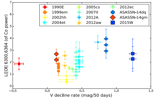
Figure D4. The [O\ I] \lambda\lambda 6300, 6364 luminosity (normalized to the ^{56}\text{Co} decay power) for the Jerkstrand et al. (2015a) sample of SNe and three objects from our sample as a function of V -band decline rate. The [O\ I] \lambda\lambda 6300, 6364 luminosities for all epochs between 200 and 500 d after explosion are plotted and are visible as multiple points for each object.
