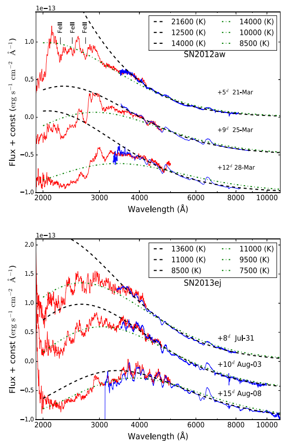
Figure 14. Early-time spectral evolution of the Type IIP SN 2012aw and the (almost) Type IIL SN 2013ej. The red portion of each spectrum corresponds to UV coverage obtained with Swift , while visual-wavelength spectra at similar epochs are plotted in blue. Blackbody fits are overplotted as dashed and dotted lines (see the text).
