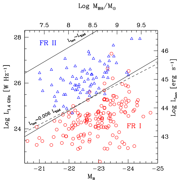
Fig. 2. The radio jet power – host optical magnitude plane with the line sharply dividing FR I from FR II (dashed line, from Ledlow & Owen 1996). According to reasonably well established correlations this plane is equivalent to an accretion power vs. black hole mass plane (right and upper axis). The central diagonal line represents L_{\text{ion}} \sim 6 \times 10^{-3} L_{\text{Edd}} .
