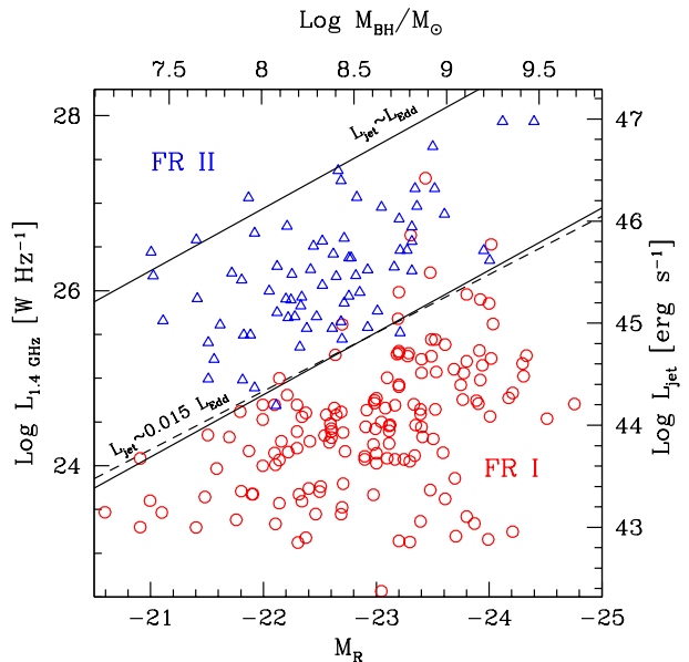
Fig. 1. The radio jet power – host optical magnitude plane with the line dividing FR I from FR II (dashed line, from Ledlow & Owen 1996). Triangles: FR II; circles: FR I. The two axes have been re-expressed as jet power vs. black hole mass (right and upper axis). The two diagonal solid lines represent L_{\text{jet}} = 0.015 L_{\text{Edd}} and L_{\text{jet}} = L_{\text{Edd}} .
