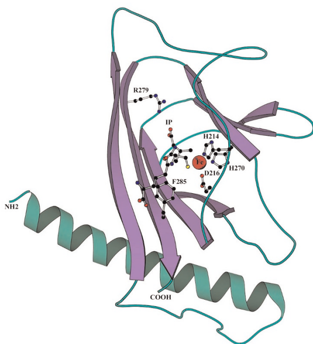
Figure 2 A structural model of the DSBH core of the 2OG-Fe(II) dioxygenase superfamily. This is based on the Emericella nidulans isopenicillin N synthase structure (PDB:lip). The side chains of the amino acid residues implicated in catalysis and in substrate binding are shown (see text) and the Fe(II) ion is indicated by a red circle.
