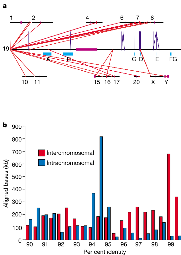
Figure 3 Recent segmental duplications on chromosome 19. a , Large ( >20 kb), highly similar ( >95\% ) intrachromosomal (blue) and interchromosomal (red) segmental duplications are shown for chromosome 19. Chromosome 19 is drawn at a greater scale relative to the other chromosomes. Gene clusters detected in duplicated sequences ( >1 kb with identity >90\% ) are represented as light blue bars below the chromosome 19 sequence. A, B, ZNF genes; C, cytochrome P450; D, pregnancy-specific \alpha -1-glycoprotein (PSG); E, chorionic gonadotropin \beta -peptide (CG \beta ); F, leukocyte immunoglobulin-like receptor; G, killer cell immunoglobulin-like receptor. b , Sequence similarity of segmental duplications. For all pairwise alignments, the total number of aligned bases was calculated and binned based on per cent sequence identity. Sequence identity distributions for interchromosomally (red) and intrachromosomally (blue) duplicated bases are shown.
