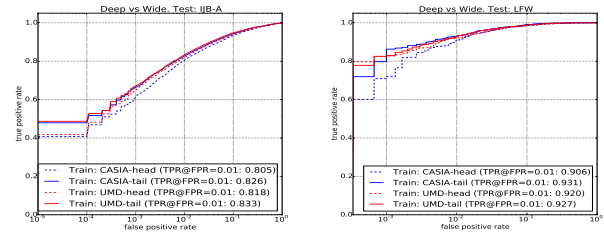
(a) IJB-A (b) LFW Figure 7: Performance on (a) IJB-A [17] and (b) LFW [12] of the networks trained on CASIA [39], and UMDFaces [2] ‘head’ and ‘tail’ sets. The performance of the networks trained on ‘tail’ are better across the range of false positive rate. (Best viewed digitally)
