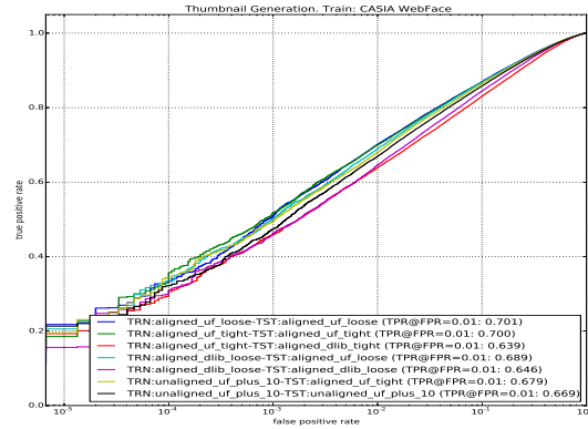
Figure 13: The performance of seven sets of train and test thumbnail generation methods with CASIA WebFace as the training set and UMDFaces batch-3 [2] as the test set. We again see that aligning both training and testing sets using [28] gives the best performance. Also, using a loose alignment gives the best performance (blue) just slightly ahead of using a tight alignment (green).
