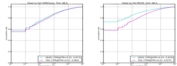
(a) UMDFaces (b) MS1M Figure 8: Performance on IJB-A [17] of ResNets trained on UMDFaces [2], and MS-Celeb-1M [7] ‘head’ and ‘tail’ sets. The ‘head’ sets are better.
