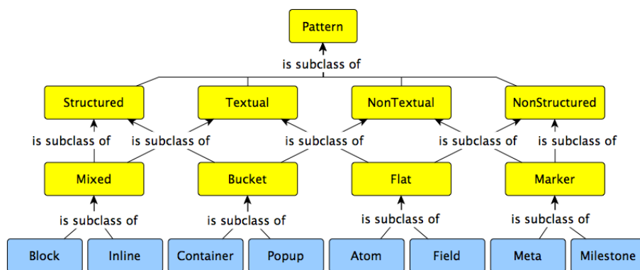
Fig. 2. A Graffoo diagram [17] describing the eight concrete patterns for document structures (bottom classes, in blue) described in [5] and [6], which are directly inspired by the OBO Foundry Principles 25 . In particular, our ontologies:
