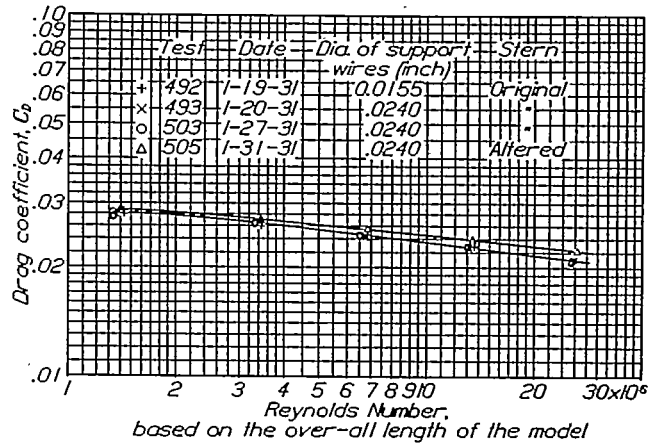
FIGURE 4.—Drag coefficients of model A
