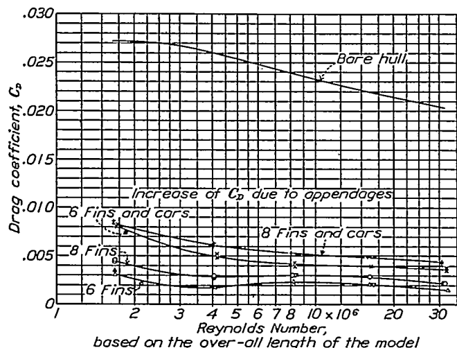
FIGURE 8.—The increase of drag coefficient of model M resulting from fins and cars
