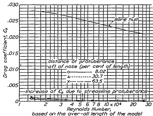
FIGURE 7.—The increase of drag coefficient of model A resulting from a streamline protuberance located in various positions along the hull
