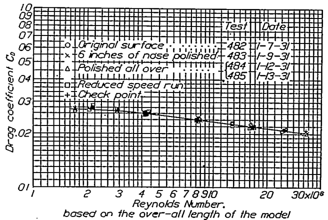
FIGURE 5.—Drag coefficients of model M
