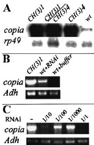
Figure 4. Parp mutations or Parp (RNAi) elevate copia transcript levels. (A) A Northern blot of total RNA from second instar larvae of the indicated genotypes was probed with copia sequences. The 5.5-kb copia transcript is overproduced up to 50-fold in CH(3)1 or CH(3)4 homozygotes, and in CH(3)1/CH(3)4 trans-heterozygotes compared to wild-type. An rp49 probe was used as a loading control. (B) Quantitative RT-PCR shows that injection of Parp -specific RNAi, but not buffer, causes copia RNA to be overproduced. Primers specific to Adh served as a loading control. (C) Copia RNA accumulation does not cause lethality. Injection of mutant CH(3)1 embryos with RNAi specific to copia suppressed the accumulation of excess copia RNA and resulted in the elimination of all copia transcripts detectable by RT-PCR within 16 h. Sequential dilutions of the RNAi gave a graded response. However, the treatment did not rescue larval lethality.
