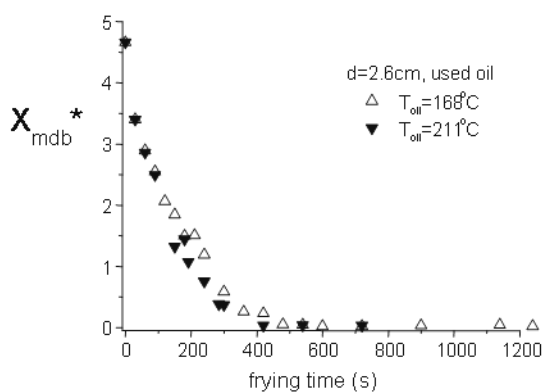
Figure 3: Drying curves for different oil temperatures (bigger cylinder, used oil)
