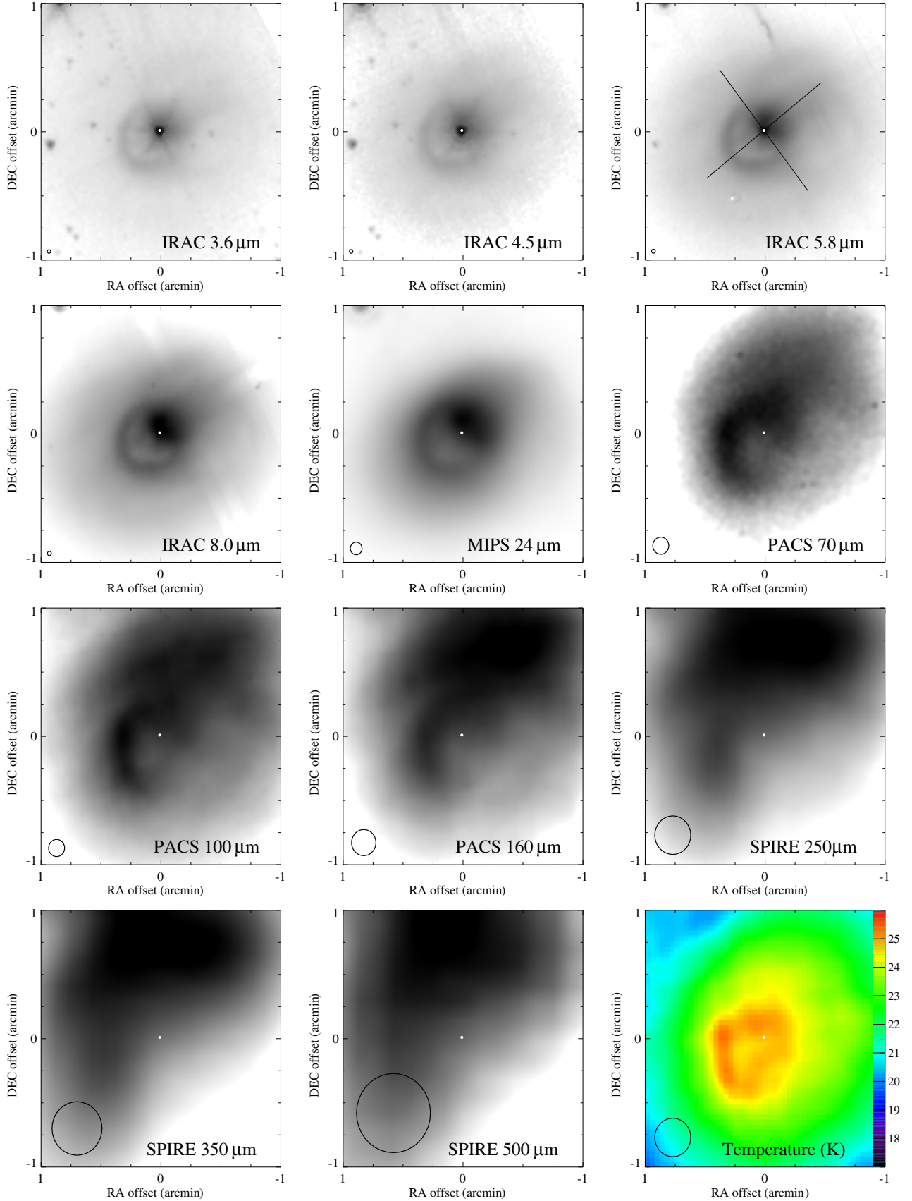
Fig. 1. Images of HD 97300 at different wavelengths. The coordinates are relative to RA_{2000} = 11^{\text{h}}09^{\text{m}}50^{\text{s}}.02 Dec_{2000} = -76^{\circ}36'47''.72 . The scaling is logarithmic. Each panel is 2' \times 2' , and north is up, east is left. The diameter of the circles in the bottom left corners corresponds to the FWHM of the PSF. The small white dot in each image indicates the stellar position. The lines in the upper right panel show the directions along which the cuts in Fig. 2 were measured. The bottom right panel shows the dust temperature on a linear scale as measured by fitting a modified black body to the 100, 160, and 250 \mu\text{m} images (see the text for details).
