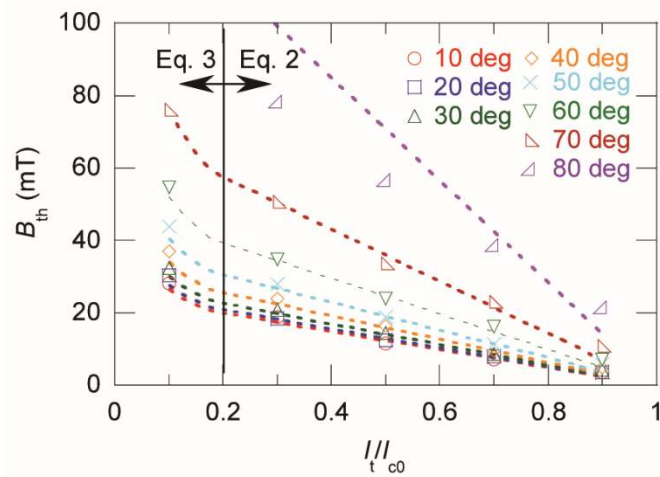
Figure 11. Experimentally-determined values for the threshold magnetic field, B_{th} obtained for various field angles, \alpha , and plotted versus the reduced transport current, i = I_t/I_{c0} . Dotted lines show calculated values using B_{th} = B_{th,\perp}/(\cos \alpha) for i \geq 0.2 (from equation 2), and B_{th} = B_{th,MB}/(\cos \alpha) for i < 0.2 (from equation 3).
