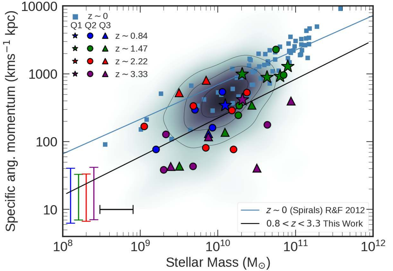
Figure 9. Specific stellar angular momentum as measured at 2R_h as a function of stellar mass. The sample coloured by spectroscopic redshift as as shown in Figure 1, and the blue shaded regions represents the KROSS z \sim 1 sample (Harrison et al. 2017). The stars represent ‘Quality 1’ targets ( V_{rot2R_h}/\sigma_{med} > 1 and \Delta PA_{im,vel}\Psi < 30^\circ ), circles ‘Quality 2’ ( V_{rot2R_h}/\sigma_{med} > 1 or \Delta PA_{im,vel}\Psi < 30^\circ ) and triangles ‘Quality 3’ galaxies ( V_{rot2R_h}/\sigma_{med} < 1 and \Delta PA_{im,vel}\Psi > 30^\circ ). The z \sim 0 Romanowsky & Fall (2012) comparison sample is shown, with the fit to the data of the form \log_{10}(j_*) = \alpha + \beta(\log_{10}(M_*/M_\odot) - 10.10) , with \alpha = 2.89 and \beta = 0.51 , whilst for KROSS ( z \sim 1 ) \alpha = 2.58 and \beta = 0.62 . Our sample appears in good agreement with other z \sim 1 samples, having lower specific stellar angular momentum for a given stellar mass than galaxies at z \sim 0 , with a \alpha = 2.41 and \beta = 0.56 . The median uncertainty on specific angular momentum at each redshift is shown in the lower left corner as well as the uncertainty of the stellar mass.
