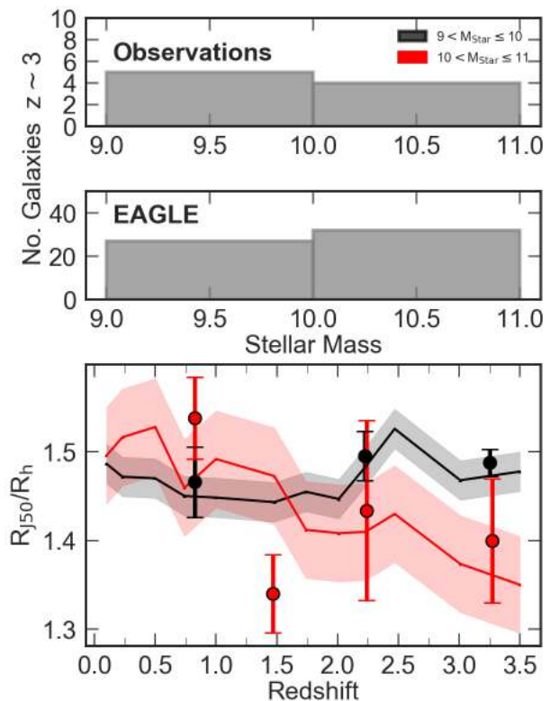
Figure 13. Top: The stellar mass distribution of our sample and EAGLE galaxies at z = 3 . Bottom: The radius ( R_{\text{J50}} ) within which 50% of the galaxies angular momentum is contained, normalised by the half-light radius of the galaxy as a function of redshift. Coloured points indicate the galaxies in our sample split into two stellar mass bins. The tracks show the median and 1\sigma evolution of EAGLE galaxies selected by stellar mass at z = 3 . For the EAGLE galaxies, we apply the stellar mass and star formation criteria at z \sim 3 and trace the galaxies back to z \sim 0.1 using the EAGLE merger trees, thus incorporating the mass evolution of galaxies. The galaxies in our sample have the mass criteria applied at their redshift and therefore shouldn't be compared directly to the tracks. We see similar evolution as the fixed mass tracks (Figure 12) with R_{\text{J50}}/R_{\text{h}} increasing by \sim 11\% from z \sim 3.5 to z \sim 0.1 . and minimal evolution in the lower stellar mass galaxies.
