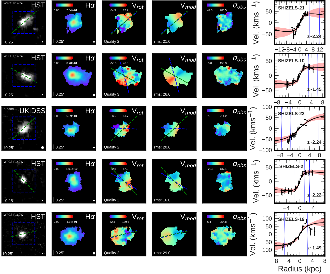
Figure 3. Example of spatially resolved galaxies in our sample. From left to right; Broadband photometry of the galaxy (left), with PA_{\text{im}} (green dashed line) and data cube field of view (blue dashed square). H\alpha or [OIII] flux map, velocity map, velocity model and velocity dispersion map, derived from the emission line fitting. PA_{\text{vel}} (blue dashed line) and PA_{\text{im}} (green dashed line) axes plotted on the velocity map and model. Rotation curve extracted about kinematic position axis (right). Rotation curve shows lines of R_h and 2R_h derived from Sérsic fitting, as well 1\sigma error region (red) of rotation curve fit (black line).
