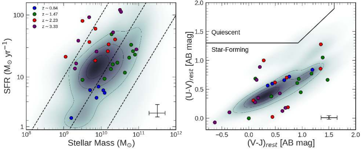
Figure 1. Left: The \text{H}\alpha and [\text{OIII}] dust-corrected star formation rate of each galaxy as function of stellar mass derived from MAGPHYS. The HiZELS sample is shown as the grey shaded region whilst our sample is coloured by redshift. Adopted 0.2 dex stellar mass uncertainty and median fractional star formation rate uncertainties are indicated by black lines. We show tracks of constant specific star formation rate (sSFR) with \text{sSFR} = 0.1, 1 and 10 \text{ Gyr}^{-1} . This shows that our sample cover a broad range of stellar mass and star formation rates, Right: The rest-frame (U - V) colour as a function of rest-frame (V - J) colour for our sample and galaxies in the HiZELS survey, demonstrating that the galaxies in our sample cover the full range of HiZELS galaxies colour-colour parameter space. Median uncertainties in (V - J) and (U - V) colour indicated by black lines. The Williams et al. (2009) boundary (black wedge) separates quiescent galaxies (top left) from star-forming galaxies (bottom right).
