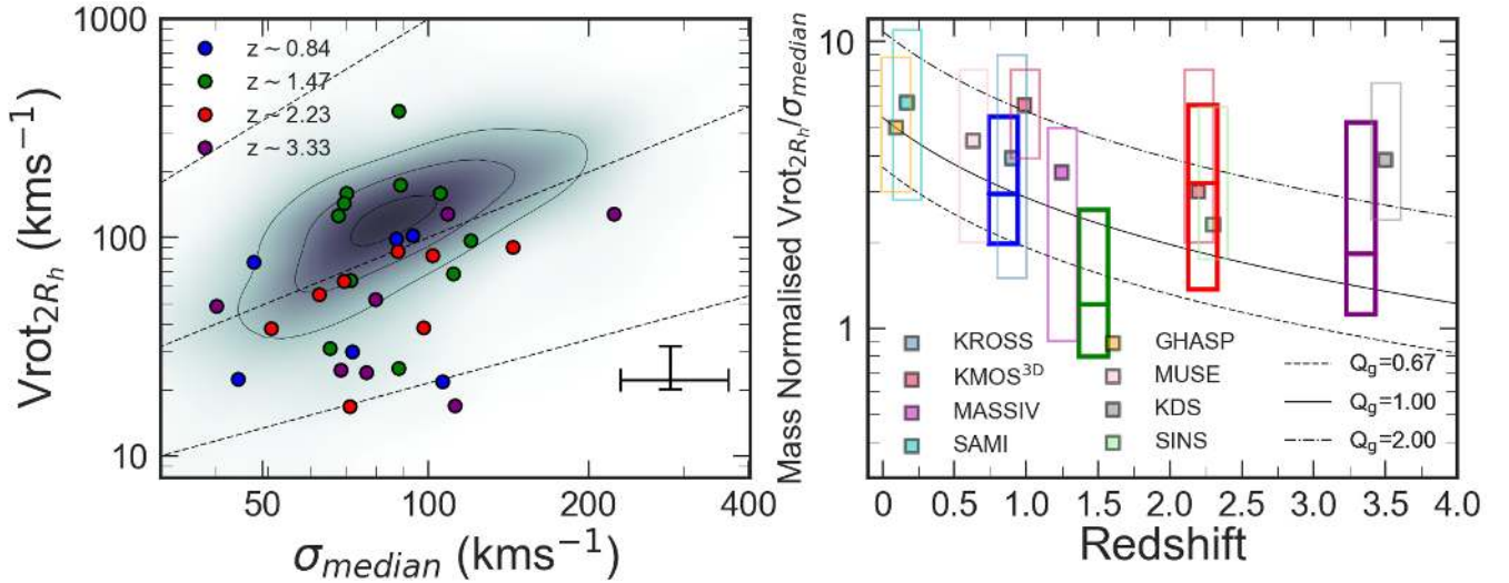
Figure 7. Left: Distribution of velocity V_{\text{rot}_{2R_h}} and \sigma_{\text{median}} in our sample, coloured by spectroscopic redshift as in Figure 1. The KROSS z \sim 0.8 survey is shown for comparison by the shaded region. Lines of 1.5V_{\text{rot}}/\sigma_{\text{median}} , V_{\text{rot}}/\sigma_{\text{median}} and V_{\text{rot}}/1.5\sigma_{\text{median}} shown for reference. Right: Mass normalised V_{\text{rot}_{2R_h}}/\sigma_{\text{median}} as function of redshift, the 16th and 84th percentile shown by the extent of the box, median as a solid line at each redshift. We also show eight comparison surveys of star-forming galaxies from 0.09 < z < 3.5 selected from the literature with median values shown by the squares. We plot tracks of V_{\text{rot}_{2R_h}}/\sigma_{\text{median}} as function of redshift, for different Toomre disk stability criterion ( Q_g ; Toomre 1964) following the procedures of Johnson et al. (2018). The majority of the sample has a mass normalised V_{\text{rot}_{2R_h}}/\sigma_{\text{median}} > 1 , with an indication of a slight evolution in the dominate dynamical support process with cosmic time, with V_{\text{rot}_{2R_h}}/\sigma_{\text{median}} increasing at lower redshift.
