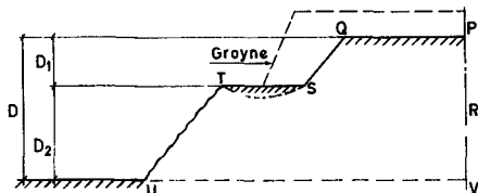
Fig 5 a Schematised profile
