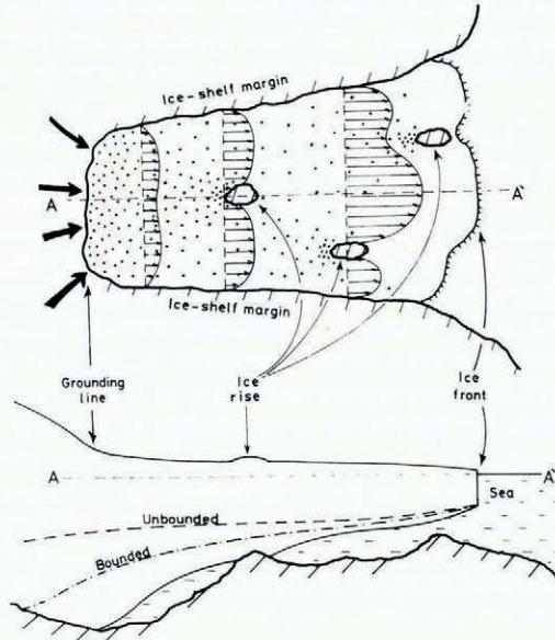
Fig. 2. A bounded ice shelf with ice rises. Velocity profiles are shown for three sections across the ice shelf. The stippling indicates the presence of a back-pressure exerted on the ice shelf by its margins and ice rises. The intensity of the stippling gives an indication of the relative magnitude of the back-pressure. Three bottom profiles are shown: the solid line is for the bounded ice shelf with ice rises and the others are for bounded and unbounded ice shelves without ice rises. The position of the grounding line is strongly dependent on the type of ice shelf that forms.
