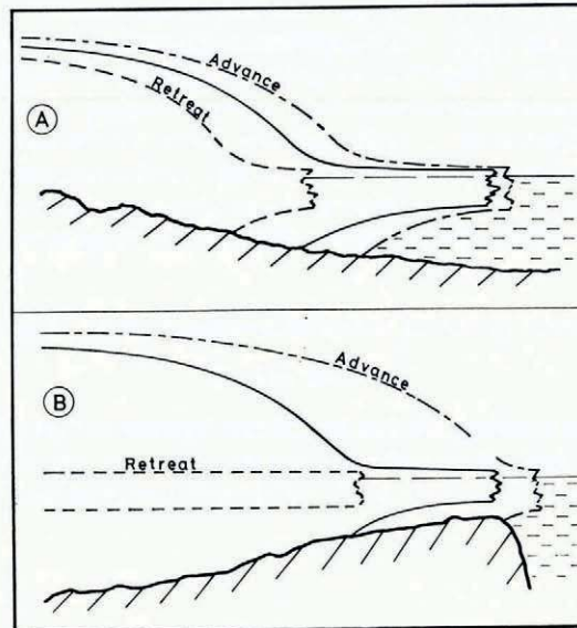
Fig. 3. Grounding-line migration. In Figure 3A the sea bed slopes down to seaward and a change in ice thickness or sea depth causes only a limited shift in the grounding-line position. If the sea bed slopes up to seaward (Fig. 3B) and the ice sheet is not protected by a bounded or partially grounded ice shelf then there are only two stable modes. These are represented by the "advance" and "retreat" profiles in Figure 3B. With a suitably bounded or pinned ice shelf, the ice sheet may adopt a stable profile that lies between these two extremes, such as that represented by the solid line. The grounding line may then migrate in response to changes in the ice shelf as well as to changes in ice thickness and sea depth.
