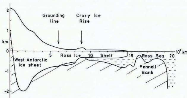
Fig. 4. A section through the West Antarctic ice sheet and across the Ross Ice Shelf (see Fig. 1). The bedrock topography is similar to that shown in Figure 3B, and the grounding line is maintained in its present position by back-pressure that is exerted on the Ross Ice Shelf by its sides and by the Crary Ice Rise. Only a very small thickening would be necessary for the ice sheet to advance to cover Crary Ice Rise. Thereafter, further advance would require grounding of the ice shelf on the shoals of Pennell Bank.
