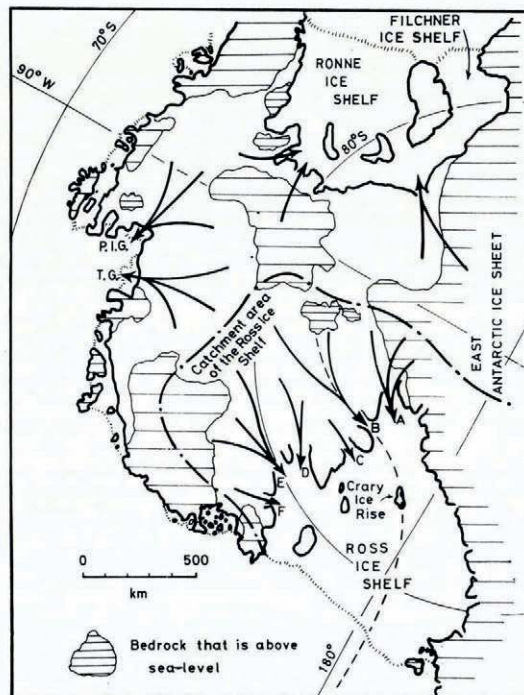
Fig. 1. West Antarctica, showing the areas of bedrock that are above sea-level. The arrows represent ice streams that drain the ice sheet. Most of the ice that flows into the Ross Ice Shelf from West Antarctica drains through ice streams B, D, and E. Pine Island Glacier (P.I.G.) and Thwaites Glacier (T.G.) carry most of the ice that drains northward. These glaciers appear to be relatively unprotected by bounded or partially grounded ice shelves. A vertical section taken along the broken line through ice stream B and the Ross Ice Shelf is shown in Figure 4.
