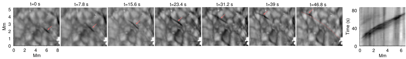
Figure 5. Time-sequence of a typical dark blob detected in the red wing at H\alpha + 0.906 \text{ \AA} ( 42 \text{ km s}^{-1} ). The blob starts from the network brightening and moves upward along the curved trajectory highlighted with the red dotted line. The corresponding t - d diagram ( right panel ) estimates an apparent propagation speed of \sim 110 \text{ km s}^{-1} .
