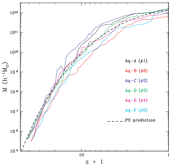
Figure 1. Mass of the most massive progenitor of each of the six Aquarius haloes as a function of redshift [ M(z) , coloured lines], compared to the extended Press–Schechter theory for a halo of mass equal to the median for the six haloes, M = 1.3 \times 10^{12} h^{-1} M_\odot (dashed line). There is over an order of magnitude variation in M(z) between the haloes at certain redshifts, even though the z = 0 masses are all within a factor of 2 (The number in brackets sorts haloes by their z = 0 mass.). The extended Press–Schechter prediction works well, but systematically overestimates the mass above z \sim 20 .
