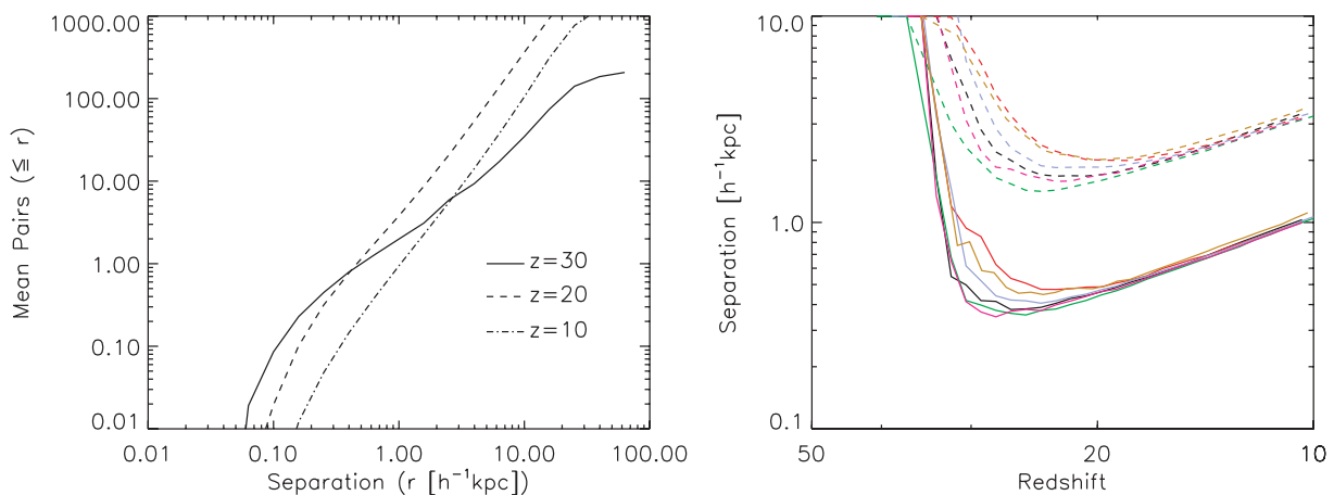
Figure 3. Clustering of Pop. III star-forming progenitor haloes. Left-hand panel: mean number of progenitor halo pairs in Aq-A, as a function of proper separation at the three redshifts indicated in the panel. Right-hand panel: mean separation of progenitor haloes in each of the six Aquarius haloes. Each halo has one neighbour within the distance given by the solid line, and 10 neighbours within the distance given by the dashed lines. Star-forming haloes have relatively nearby companions, indicating that feedback effects could be important (see text). The linear rise in separation between substructures below z \sim 20 is because the proto-halo region is still expanding with the Hubble flow at this early time.
