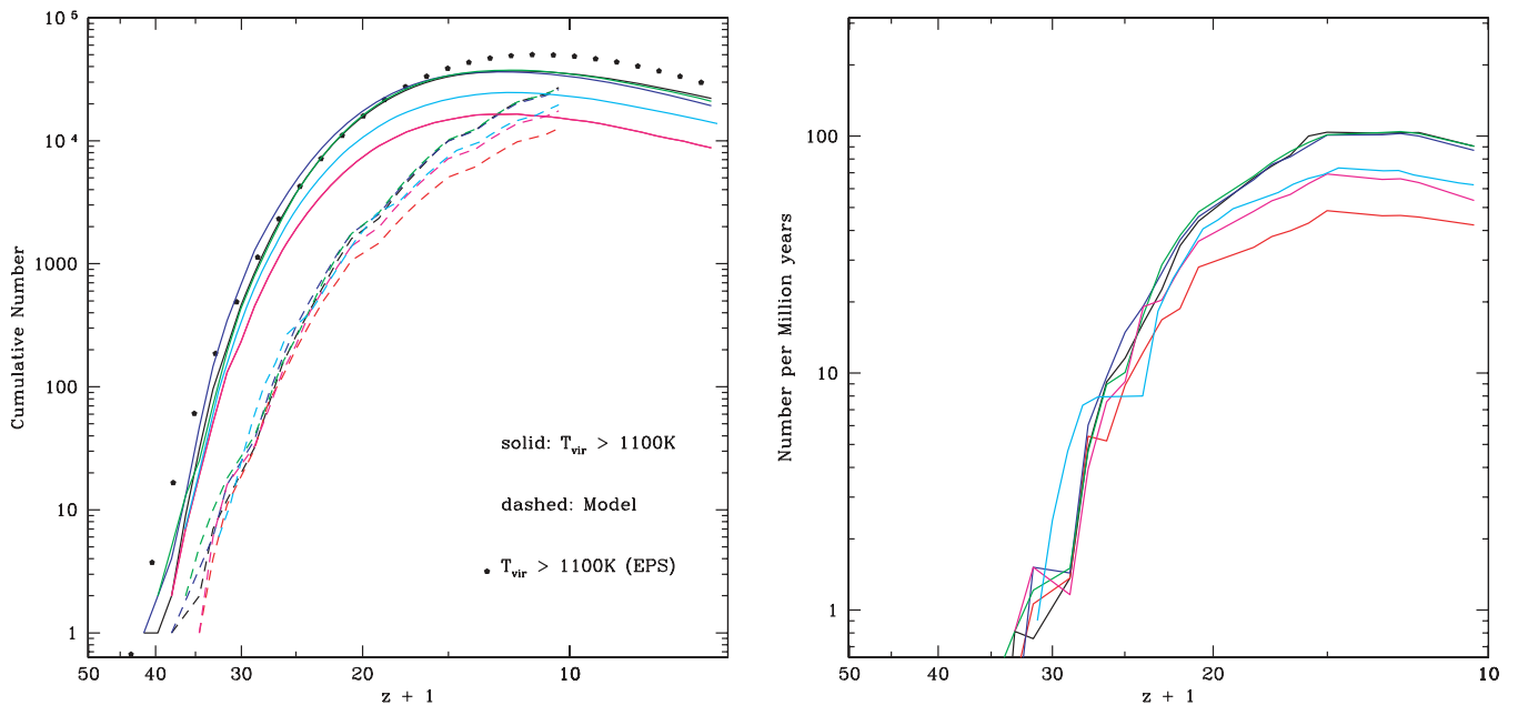
Figure 2. Pop. III star formation in galaxy halo progenitors as a function of redshift. Left-hand panel: cumulative number of progenitor haloes with virial temperature above 1100 K for each of the six Aquarius haloes (colour solid lines). The black dots show the extended Press–Schechter prediction which works well, but increasingly overestimates the number of haloes after z \sim 15 . Gas in such haloes is hot enough for significant \text{H}_2 formation. The dashed lines show the cumulative number of independent sites of Pop. III star formation according to the model of Gao et al. (2007) which, in addition to a virial temperature criterion, takes the merger history of the halo into account. This more stringent criterion reduces the number of forming stars; yet a Milky Way-type halo still had several hundreds of Pop. III star-forming progenitors at redshift z = 25 and \sim 10^4 at z = 10 . The halo-to-halo variation is large, a factor of \sim 5 at z = 10 . The cumulative number of haloes drops after z \sim 10 as haloes begin to merge. Right-hand panel: the star formation rate. The rate increases from a few star forming events per Myr at z = 30 , to several tens at z = 20 and changes little thereafter.
