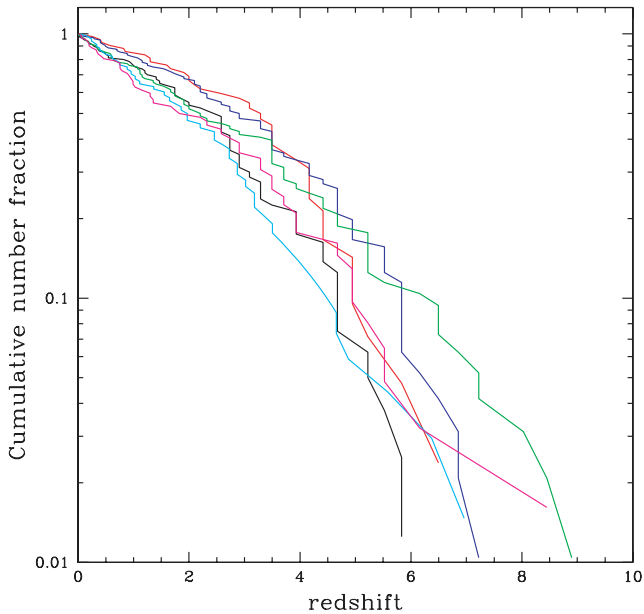
Figure 11. Cumulative fraction of first galaxy haloes that were accreted before a given redshift and survive until z=0 . The different lines correspond to the six Aquarius haloes. Typically 50 per cent of haloes fell in before z=3 .
