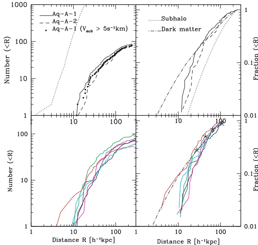
Figure 12. Left-hand panels: present-day cumulative number of first galaxy halo remnants (i.e. substructures whose progenitors had T_{\text{vir}} > 10^4 K at z = 10 ), as a function of distance, R , from the centre of the main halo. In the top panel, the solid line shows all haloes in Aq-A-1, the thick dotted line haloes with V_{\text{max}} > 5 \text{ km s}^{-1} in Aq-A-1 and the dashed lines all haloes in Aq-A-2. Haloes with V_{\text{max}} < 5 \text{ km s}^{-1} are not resolved in Aq-A-2; for V_{\text{max}} > 5 \text{ km s}^{-1} the distributions in the two simulations agree within the noise. The thin dotted lines shows the cumulative number of all substructures with V_{\text{max}} > 2 \text{ km s}^{-1} which is almost two orders of magnitude higher than the number of first galaxy remnants. The bottom panel shows results for all five level-2 haloes. Top right panel: as the left-hand panels, but showing the cumulative fraction normalized to the number within the virial radius, for Aq-A-1 (thin solid line) and Aq-A-2 (dashed line). Bottom right panel: as the left-hand panels, but showing the cumulative fraction within R = 120 h^{-1} \text{ kpc} for all five Aquarius haloes. The black solid lines in the top and bottom panels indicate the dark matter profile and the dotted line in the top panel the radial profile of all substructures. The pentagons in the lower panel correspond to known Milky Way satellites. Their radial distribution resembles that of the outer first galaxy remnants.
