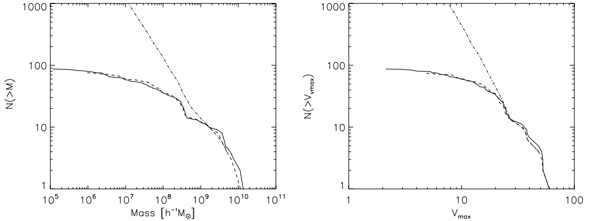
Figure 9. Left-hand panel: cumulative mass function at z = 0 of ‘first galaxy’ haloes (i.e. bound substructures which had a progenitor at z > 10 with T_{\text{vir}} > 10^4 K), for the Aq-A-1 (solid line) and the 8\times lower resolution Aq-A-2 (dashed line) simulations. Numerical convergence is very good above 100 particles (corresponding to 10^6 h^{-1} M_{\odot} in Aq-A-2). For comparison, the dashed-dotted line is the z = 0 mass function of all gravitationally bound substructures in Aq-A-1. Right-hand panel: as the left-hand panel, but for the maximum of the circular velocity curve, V_{\text{max}} .
