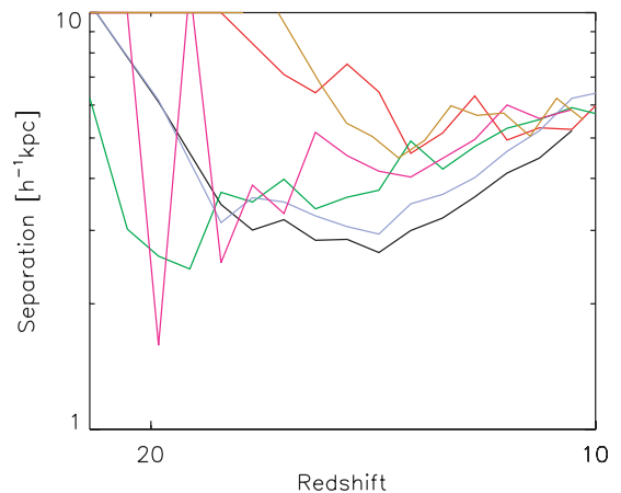
Figure 5. Clustering of ‘first galaxy’ progenitor haloes (virial temperature, T_{\text{vir}} > 10^4 K). Left-hand panel: mean number of progenitor halo pairs in Aq-A, as a function of proper separation, at the redshifts indicated in the panel. Right-hand panel: redshift evolution of the mean separation between pairs of haloes with T_{\text{vir}} > 10^4 K. By z = 10 , the mean separation between first galaxy haloes is \sim 6 h^{-1} kpc and each halo has on average another 10 haloes within \sim 20 h^{-1} kpc. The typical distance to a neighbouring halo has a large scatter amongst realizations, reflecting the fact that these haloes only just began to form at these early times.
