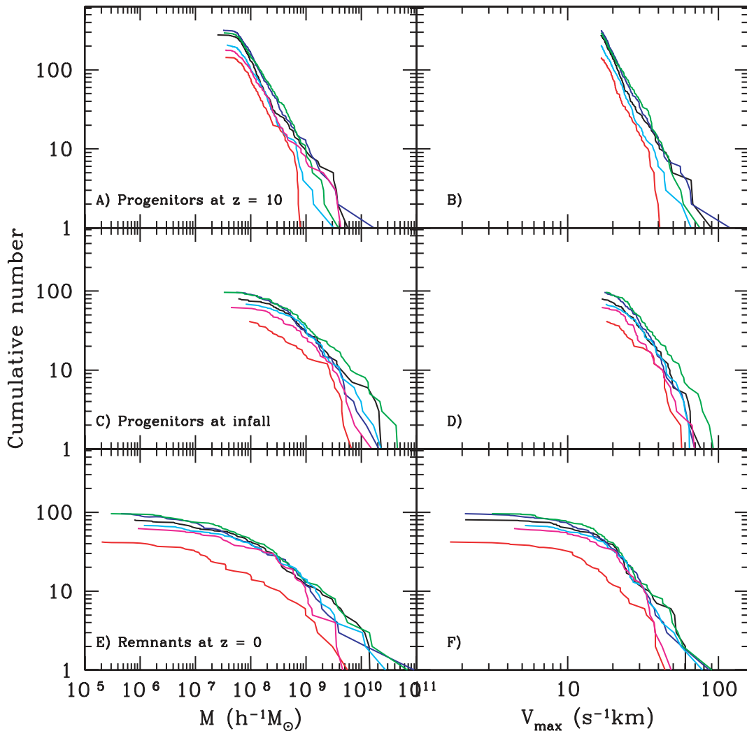
Figure 10. Statistics of first galaxy haloes in all six Aquarius haloes (the colour scheme is as in Fig. 1) at z = 10 (top), when they are accreted by the main halo (middle), and at z = 0 (bottom). The left-hand panels show cumulative mass functions and the right-hand panels show cumulative V_{\max} distributions. There is a large variance between the different Aquarius haloes at all redshifts. For example, the mass of the most massive z = 0 remnant varies between 3 \times 10^9 h^{-1} M_{\odot} and nearly 10^{11} h^{-1} M_{\odot} . The more massive Aquarius haloes tend to have the more massive substructures. Comparing the z = 0 masses with those at infall or at z = 10 demonstrates that most substructures lose a considerable fraction of their mass by the present.
