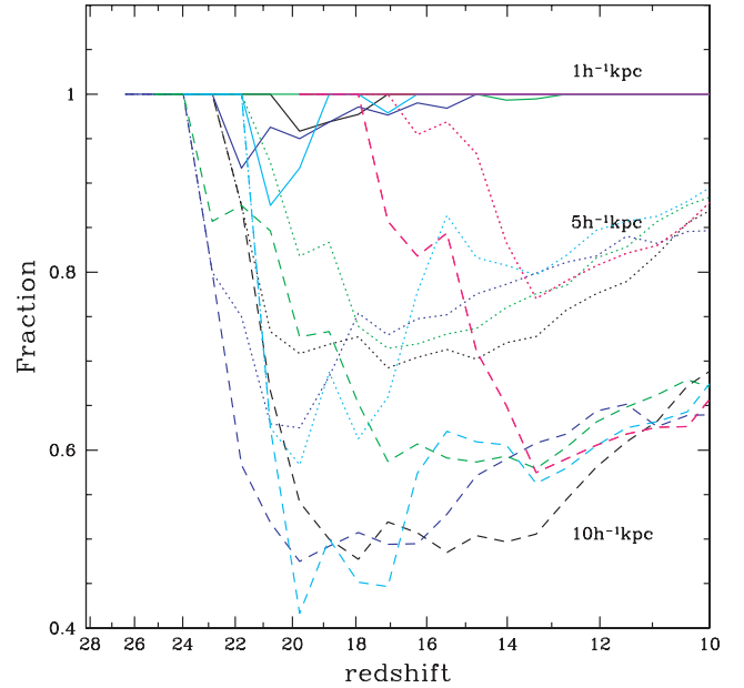
Figure 6. Fraction of first galaxies not affected by neighbouring first galaxies as a function of redshift, if the radius of influence of the feedback is R = 10, 5 or 1 h^{-1} kpc (dashed, dotted, and solid lines, respectively). For the smaller value of R , feedback has little or no effect, but for larger R , feedback may decrease the number of first galaxies considerably, up to a factor of \sim 2 .
