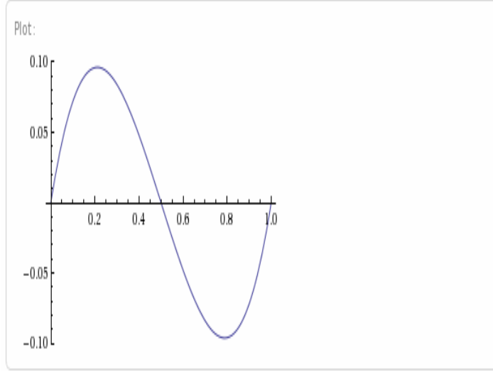
Figure 2: Dynamics with cultural substitution in Bisin and Verdier (2001): \dot{q}^i as a function of q^i .
