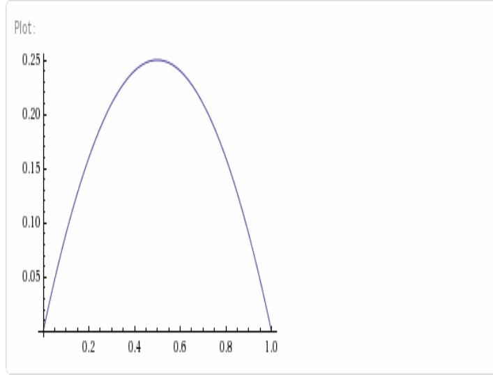
Figure 1: Dynamics with cultural substitution in Cavalli Sforza and Feldman (1981): q^i as a function of q^i .
