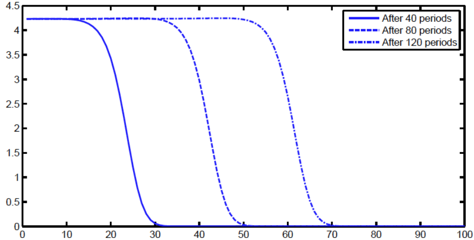
Figure 3: Stationary constant traveling wave: Each curve represents the wave at a time t , with the variable l on the x -axis
