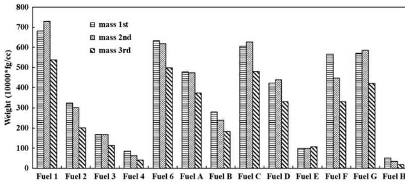
Figure 12. Particulates measured for fuels at size of \sim 27 nm.
