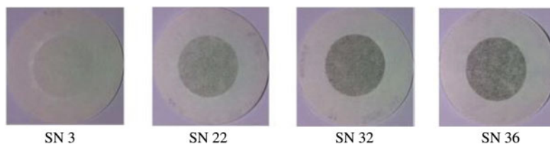
Figure 6. Actual pictures of Whatman no. 4 filter paper with varying SAE smoke number.
