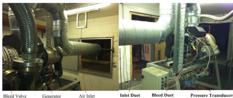
Figure 3. Gas turbine experimental set-up.
