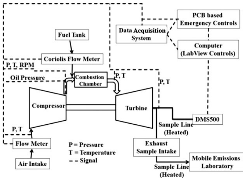
Figure 2. Experimental set-up.
