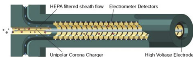
Figure 5. Principle of particulate emission measurement instrument (DMS 500) (43) .
