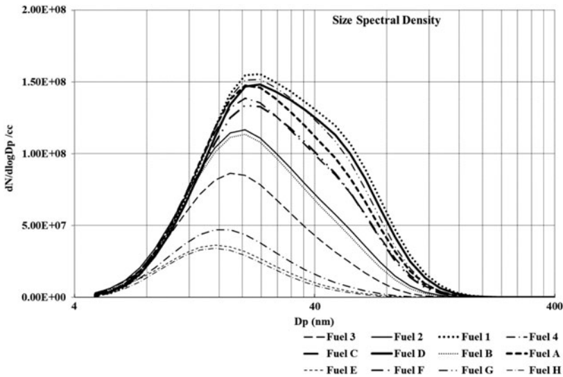
Figure 11. Number and size distribution of particulates measured for 3 rd condition.
