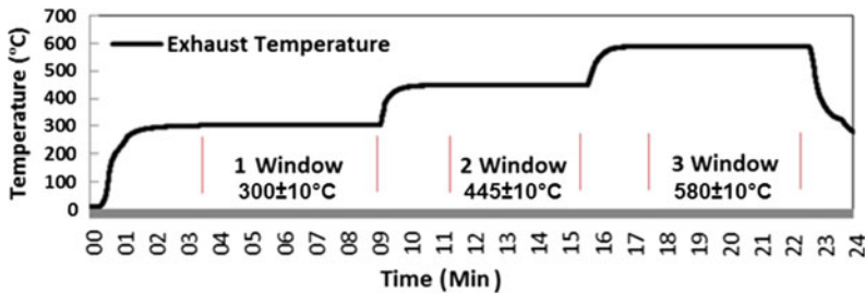
Figure 7. Exhaust temperature profile for illustration of engine test windows.
