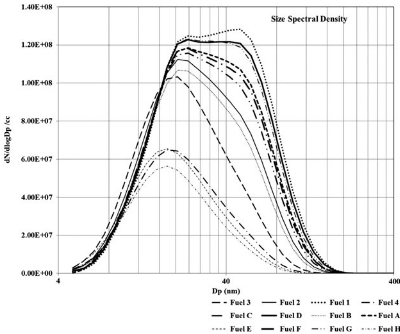
Figure 9. Number and size distribution of particulates measured for 1 st condition.
