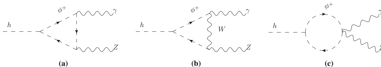
Fig. 2 Examples of one-loop diagrams contributing in the FG to the h \rightarrow \gamma Z process whose renormalization gives rise to a contribution proportional to an anomalous Higgs self-coupling
