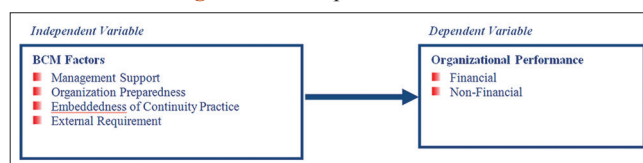
Figure 2: Conceptual framework
