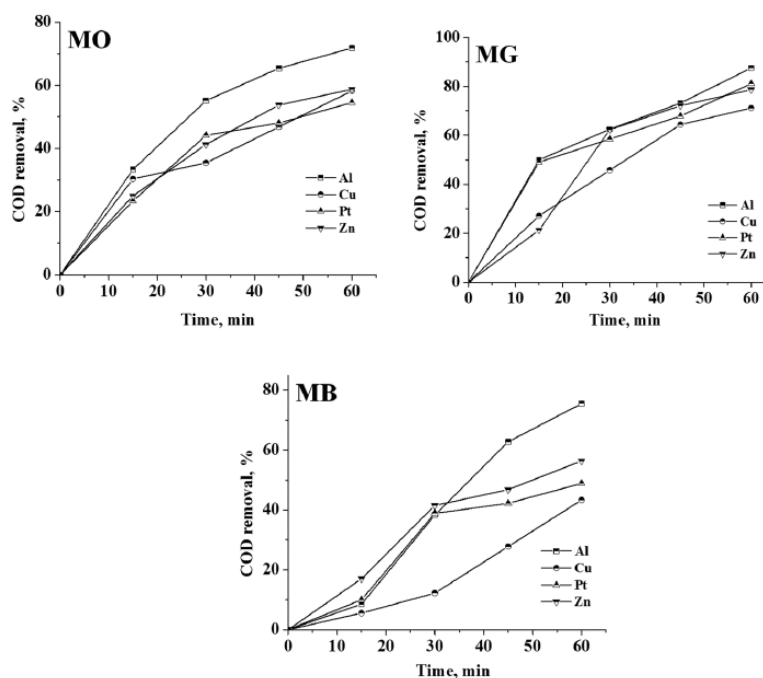
Figure 6. Percentage of COD removal with time on different cathode materials.
