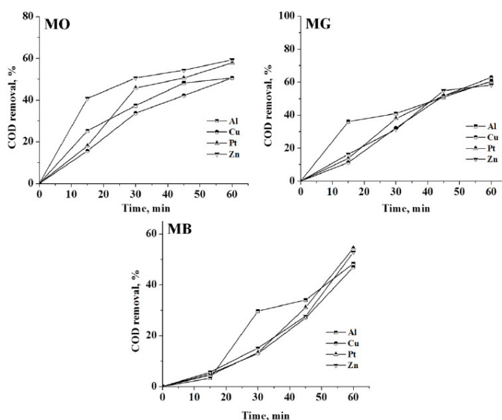
Figure 8. Percentage of color removal in the anode compartment of the divided cell system.
