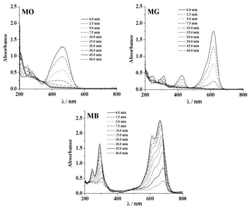
Figure 4. The UV-Visible absorption spectra with time of electrolysis using Pt anode and Al cathode.
