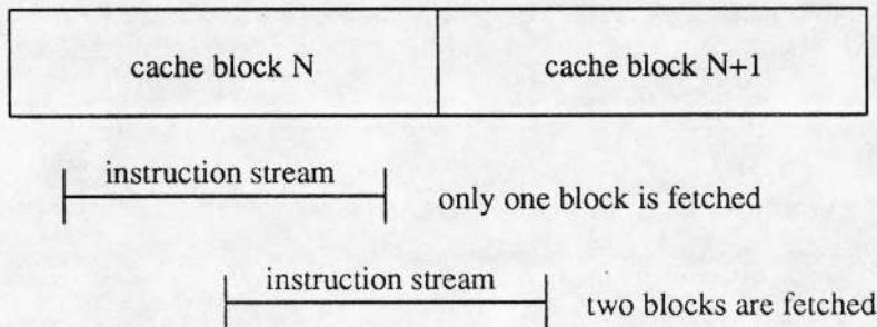
Figure 14: Reference stream and cache block refills.
