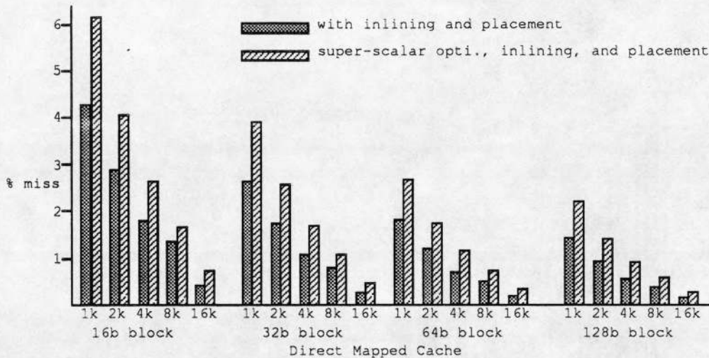
Figure 10: Effect of superscalar optimizations for direct mapped cache.
