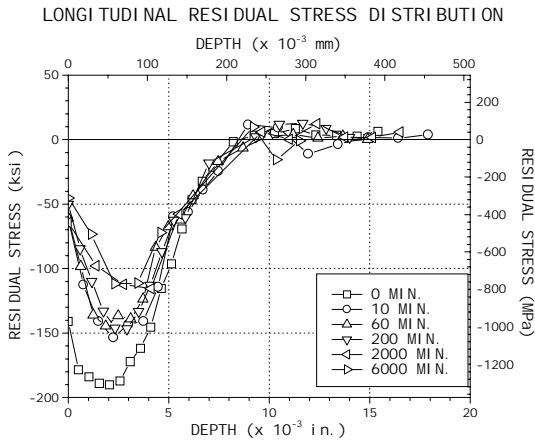
Figure 4 - Effect of exposure time at 525C on residual stress distributions in shot peened (10A, 200%) IN718.
