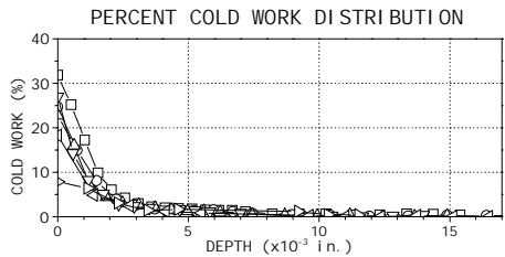
Figure 6 - Effect of exposure time on residual stress distributions in shot peened (10A, 200%) IN718 at 600C.
