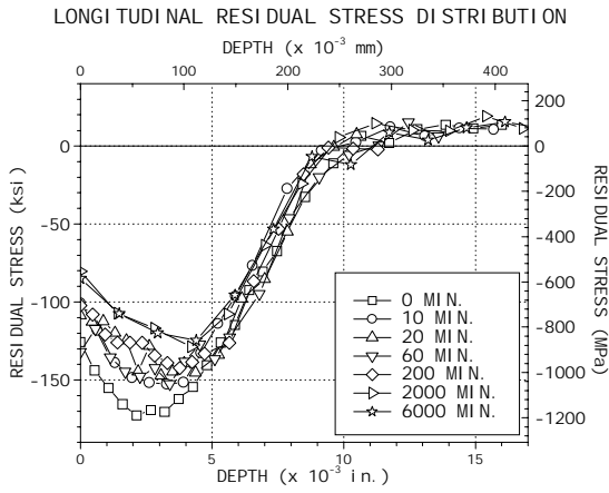
Figure 5 - Effect of exposure time on residual stress distributions in gravity peened IN718 at 525C.
