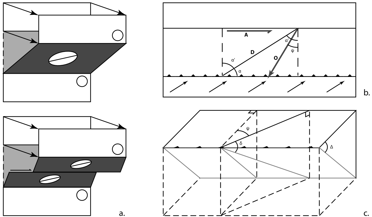
Figure 1. (a) Transpression without and with strain partitioning (modified from Tikoff and Teyssier [1994], with permission from Elsevier). (b, c) Oblique convergence D at an angle \alpha to the plate boundary is partitioned into along-strike displacement A on a vertical fault at the back and slip at a higher angle to the plate boundary O on an inclined fault plane at the front.
