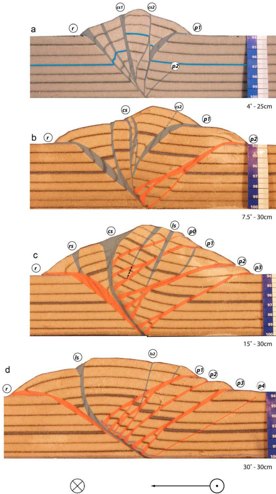
Figure 10. Effect of changing convergence angle on geometry. Cross sections for (a) 4°, (b) 7.5°, (c) 15°, and (d) 30° models (location in Figure 9).
