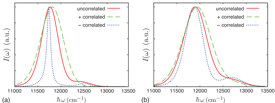
FIG. 2. Spectra of a dimer with uncorrelated, “+”-correlated, and “-”-correlated bath fluctuations without static disorder (a) and with static disorder (b).
