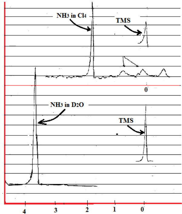
Figure 10. NMR of ammonia in \text{D}_2\text{O} and \text{CCl}_4 From Brazier [75]
