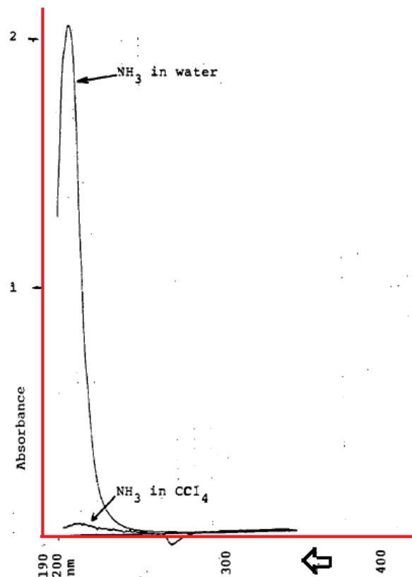
Figure 11. UV Spectra of ammonia in \text{D}_2\text{O} and \text{CCl}_4 solvents. From Brazier [75]
