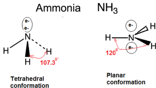
Figure 12. Alternative molecular configurations of ammonia
