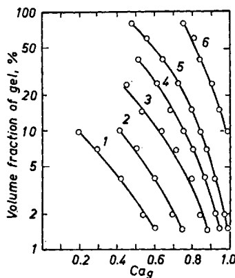
Fig. 8. Volume fraction of gel as a function of Ca_g at different concentrations of free cations (calculated from Fig. 3). (Ca_1 + Na_1) : 1 = 1.0 N; 2 = 0.5 N; 3 = 0.2 N; 4 = 0.1 N; 5 = 0.05 N; 6 = 0.01 N.
