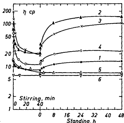
Fig. 7. Thixotropic properties of 0.2 % solutions of sodium-calcium alginates containing 0.01 N of free cations. Alginate from A. nodosum , Flakk 15/8-62, [\eta] = 10 . Ca(NO_3)_2 : 1 = 0.003 N; 2 = 0.004 N; 3 = 0.005 N; 4 = 0.006 N. 5 = Dissolved mixed sodium calcium alginate with Ca_g = 0.1 . 6 = Sodium alginate.
