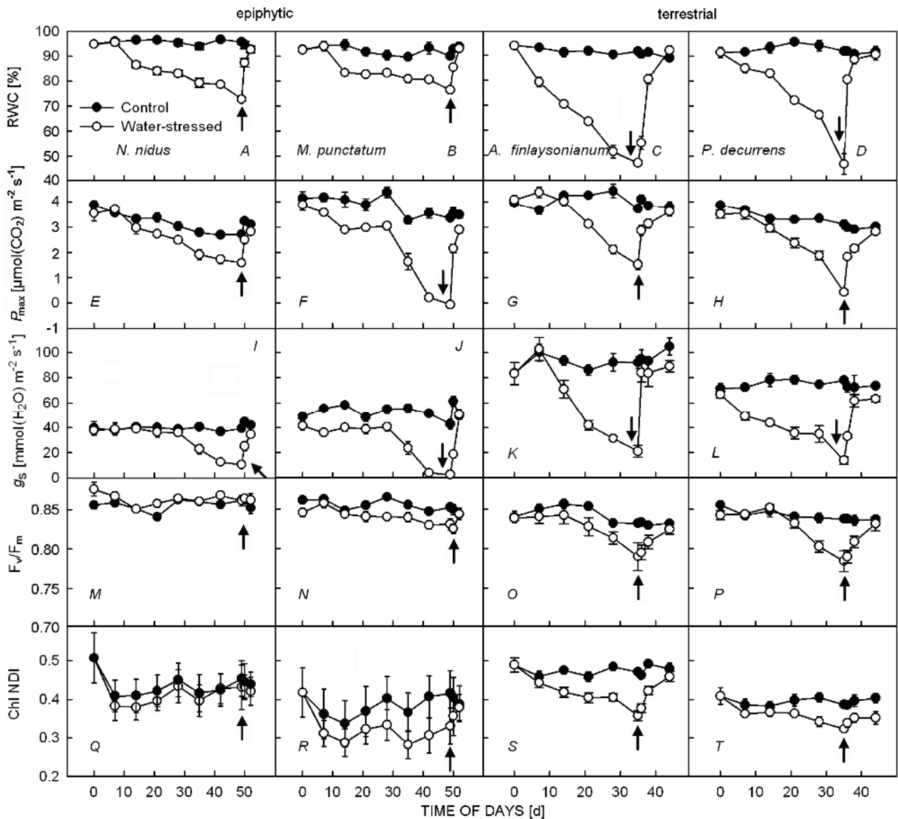
Fig. 1. The changes in leaf relative water content (RWC), net photosynthetic rate ( P_{max} ), stomatal conductance ( g_s ), and F_v/F_m at predawn and chlorophyll normalized difference index (Chl NDI) in the four fern species during the water stress and recovery periods. Arrow indicates re-watering. Means \pm SE of six plants of each species.
