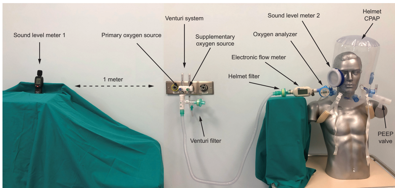
Fig. 1. Experimental setup.
