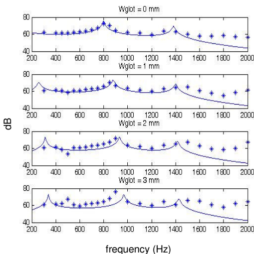
Figure 3: Measured (*) and theoretical (solid line) transfer function from glottis to lips for various glottal widths. The theoretical transfer function based to a duct of length 20 cm, terminated at lips as described above from the measurements on the mechanical model, are shown in Figure 3 as the data points (*).
