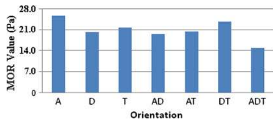
Fig. 5 Average MOR values for three-point bend testing (Pa)
