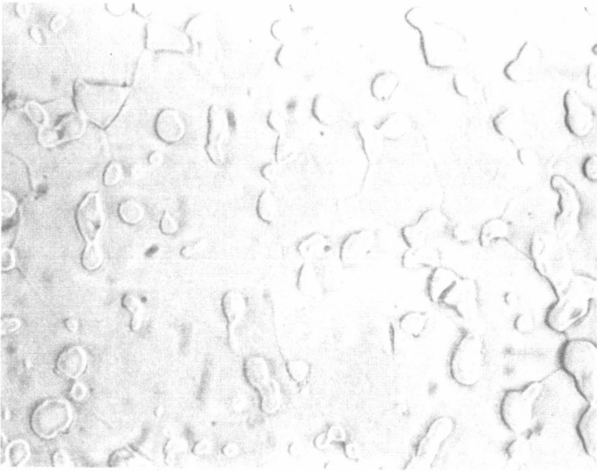
Figure 2. Steel 81M Double-Quenched-and-Tempered. Last Temper at 450C.
