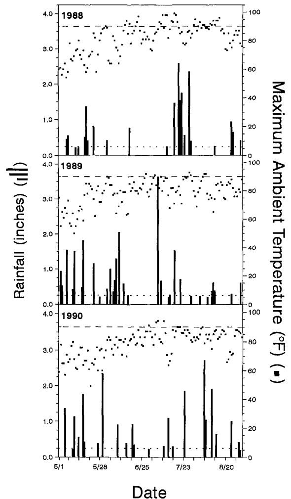
Figure 1. Daily rainfall and maximum daily air temperatures during the growing seasons of 1988, 1989, and 1990, recorded at a weather station three miles from the study site in East Brunswick, NJ.
