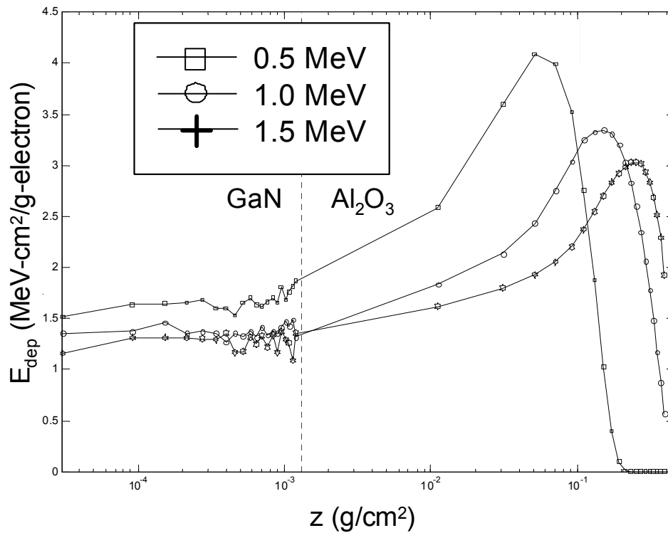
Figure 6. Dose deposition profiles for GaN (2 µm) on Al 2 O 3 (1 mm) for particle energies of 0.5, 1.0, and 1.5 MeV. Calculation was performed using 200,000 histories in 20 batches in TIGER [31].
