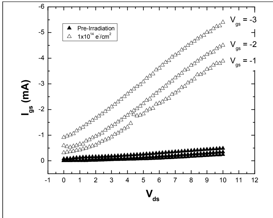
Figure 30. The pre- and post-irradiation measurements of sample A08 showing the increase in both I_{\text{drain}} (a) and I_{\text{gs}} (b) following irradiation. The curve for V_{\text{gs}} = -1 V is shown with and without I_{\text{gs}} . The irradiation and measurements were performed at liquid nitrogen temperatures ( \sim 85 K).
