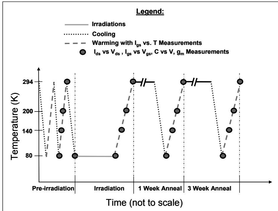
Figure 52. Experimental procedure of the second neutron irradiation experiment showing irradiations, measurements, and temperature profile.
