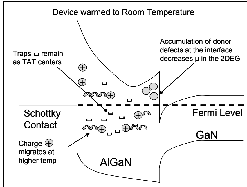
Figure 77. HFET band diagram illustrating the movement of positive charge and the accumulation of donor-like charged defects near the AlGaIn-GaN interface during post-irradiation annealing at room temperature.
