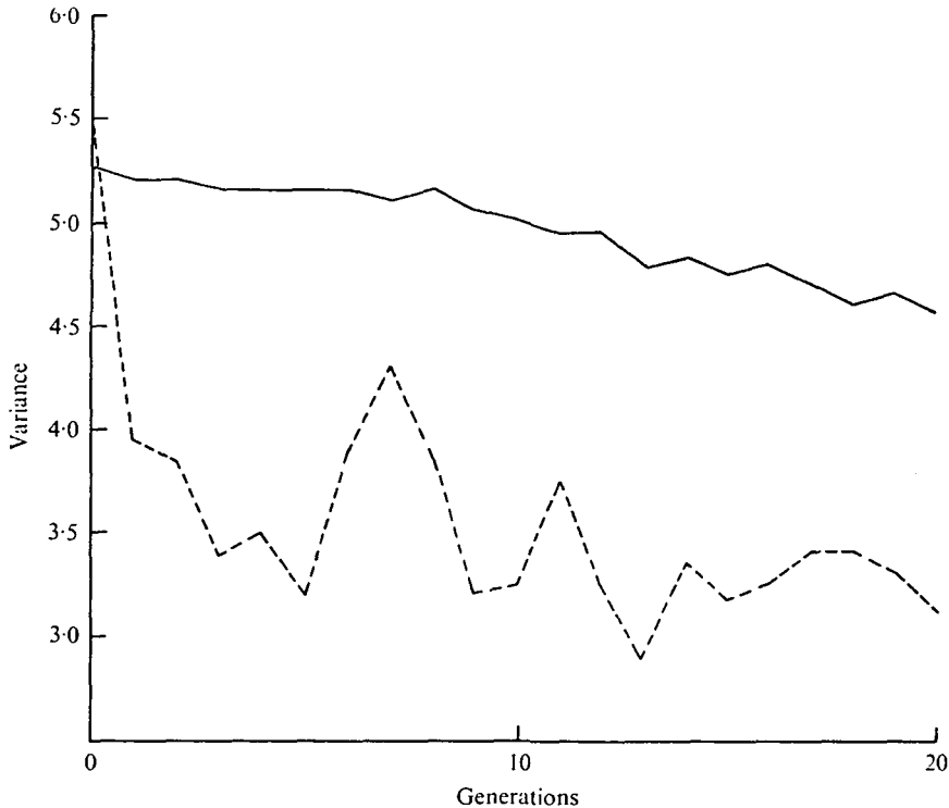
Fig. 2. Genic variance (solid) and genotypic variance (dotted) for the mouse stabilizing rank simulation.
