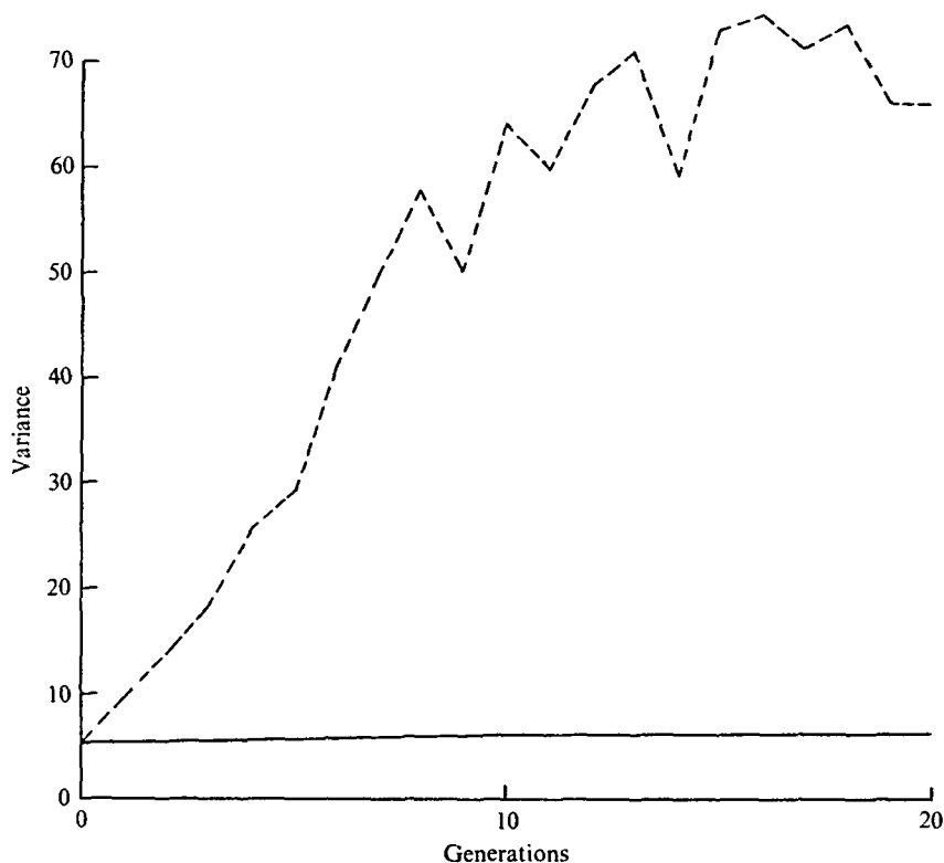
Fig. 3. Genic variance (solid) and genotypic variance (dotted) for the mouse disruptive rank simulation.
