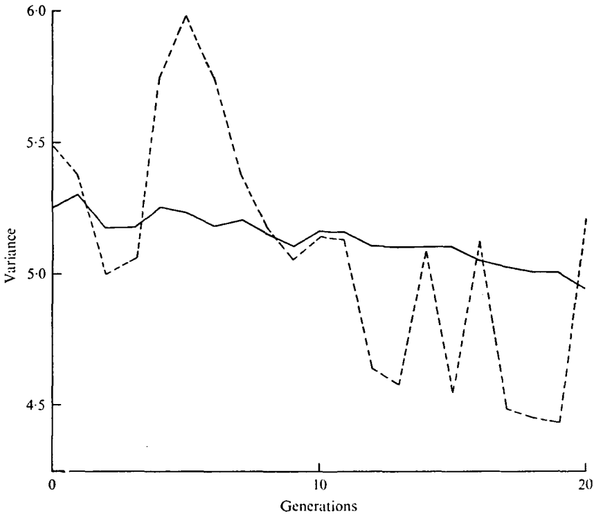
Fig. 1. Genic variance (solid) and genotypic variance (dotted) for the first mouse control simulation.
