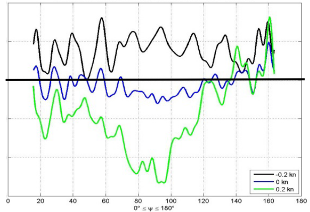
Fig. 9 Longitudinal force acting on the moored ship COU due to swinging of COW (10% ukc -12.5°/min). Wide Saeftinge dock. Influence of sway speed (positive is towards COU).
