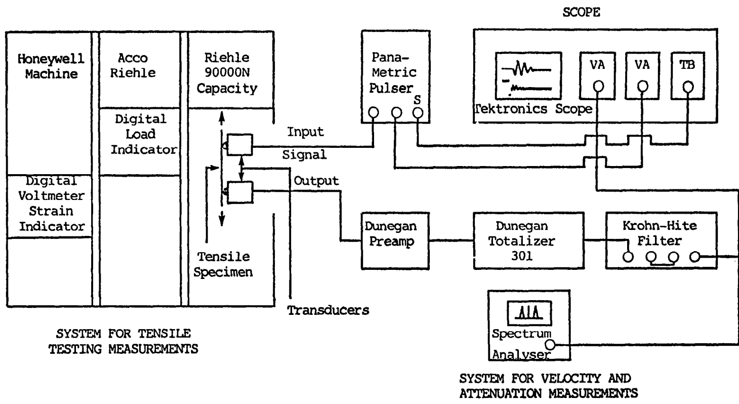
FIG. 3 -- EXPERIMENTAL SYSTEM-1
