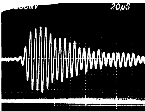
FIG. 5 - ULTRASONIC PULSE ATTENUATION VERSUS LOAD of the 150 KHZ in the Time Domaine
